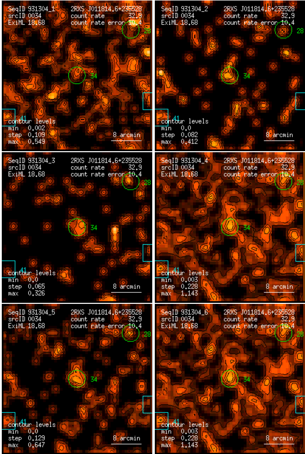
Figure 34: RASS 931304: detection 0034: band rate images, Gaussian filter: (1) PSPC channels 11 – 41, (2) 52 – 90, (3) 91 – 201, (4) 11 – 235, (5) 52 – 201, (6) 11 – 201. Broad band rates in counts/ks. Band rate contour levels in counts/ks/arcmin 2 .
