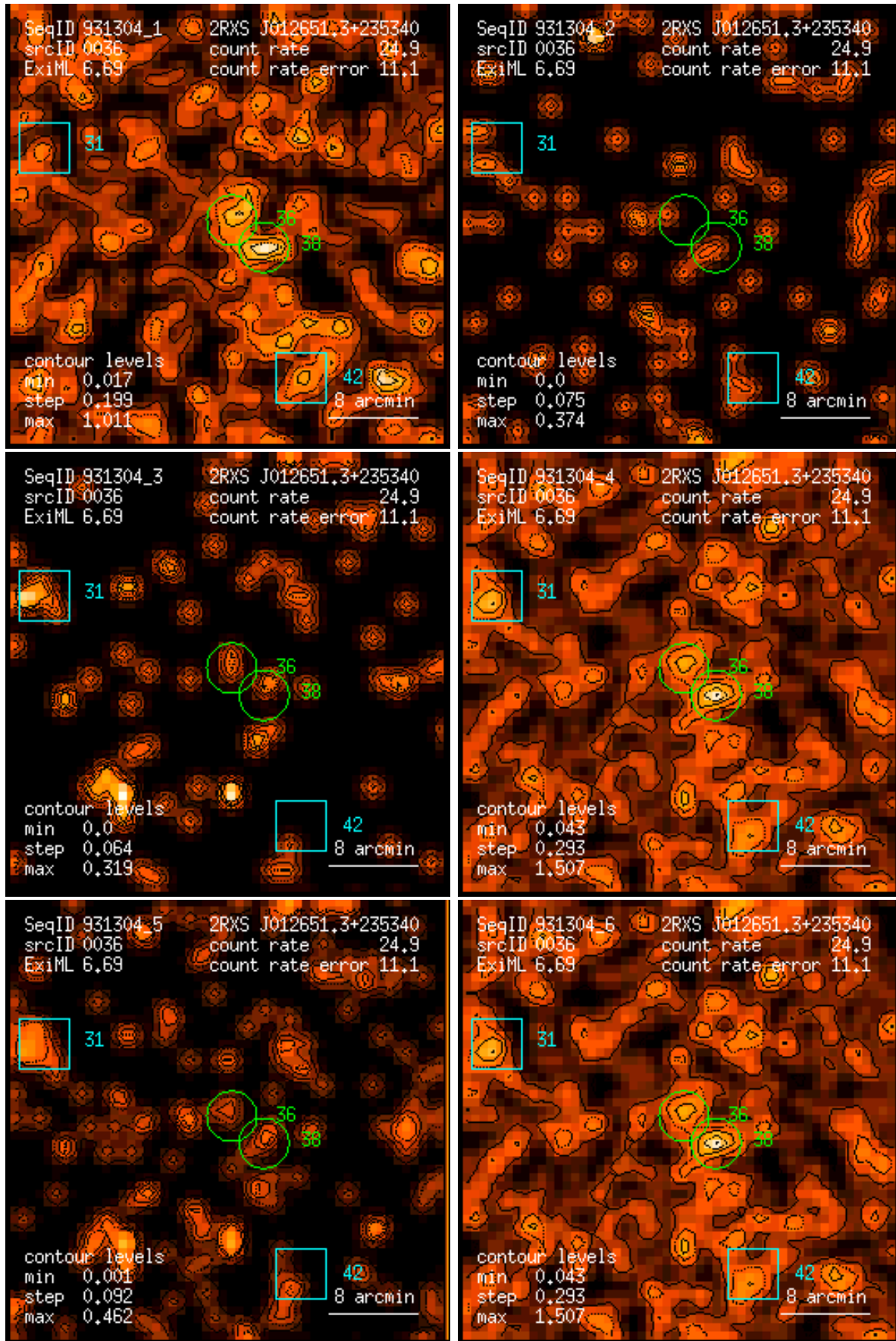
Figure 36: RASS 931304: detection 0036: band rate images, Gaussian filter: (1) PSPC channels 11 – 41, (2) 52 – 90, (3) 91 – 201, (4) 11 – 235, (5) 52 – 201, (6) 11 – 201. Broad band rates in counts/ks. Band rate contour levels in counts/ks/arcmin 2 .
