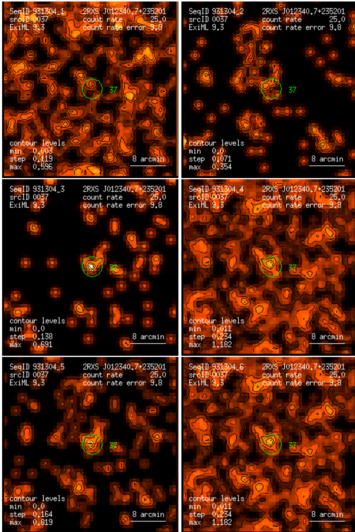
Figure 37: RASS 931304: detection 0037: band rate images, Gaussian filter: (1) PSPC channels 11 – 41, (2) 52 – 90, (3) 91 – 201, (4) 11 – 235, (5) 52 – 201, (6) 11 – 201. Broad band rates in counts/ks. Band rate contour levels in counts/ks/arcmin 2 .
