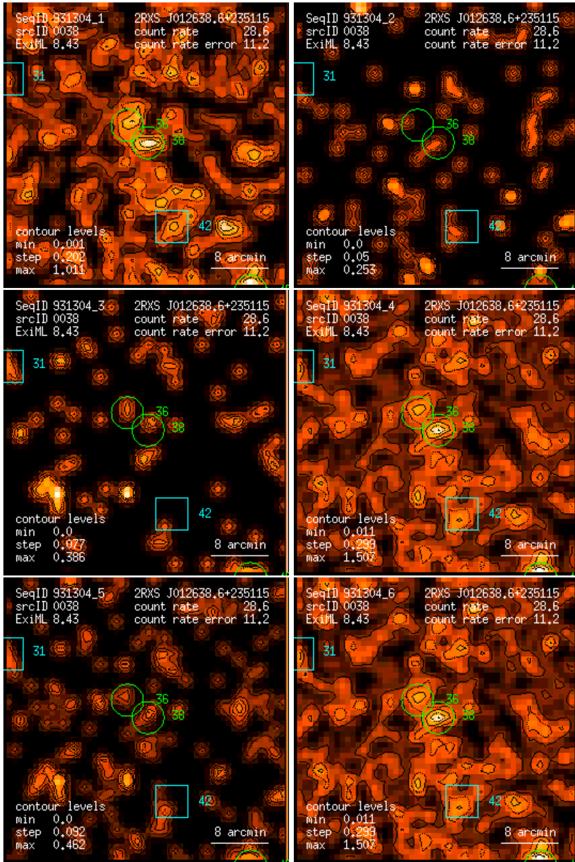
Figure 38: RASS 931304: detection 0038: band rate images, Gaussian filter: (1) PSPC channels 11 – 41, (2) 52 – 90, (3) 91 – 201, (4) 11 – 235, (5) 52 – 201, (6) 11 – 201. Broad band rates in counts/ks. Band rate contour levels in counts/ks/arcmin 2 .
