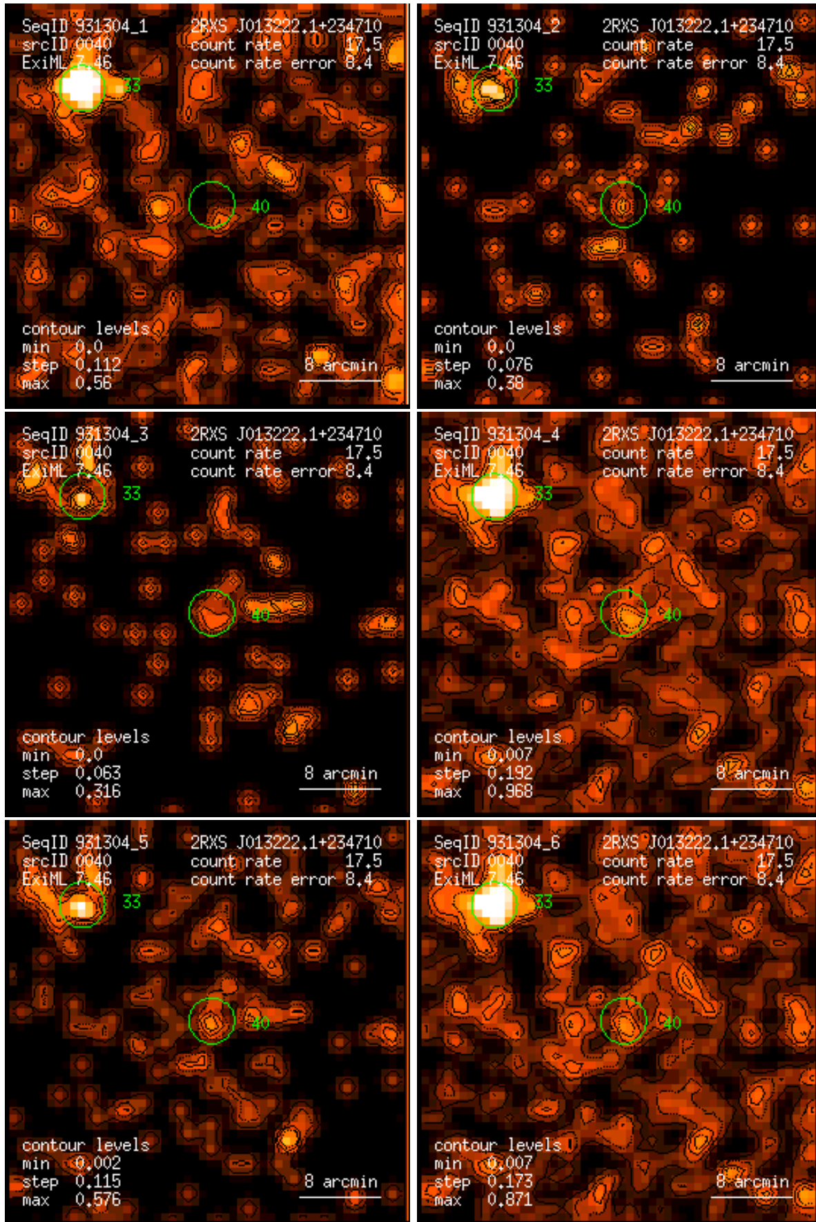
Figure 40: RASS 931304: detection 0040: band rate images, Gaussian filter: (1) PSPC channels 11 – 41, (2) 52 – 90, (3) 91 – 201, (4) 11 – 235, (5) 52 – 201, (6) 11 – 201. Broad band rates in counts/ks. Band rate contour levels in counts/ks/arcmin 2 .
