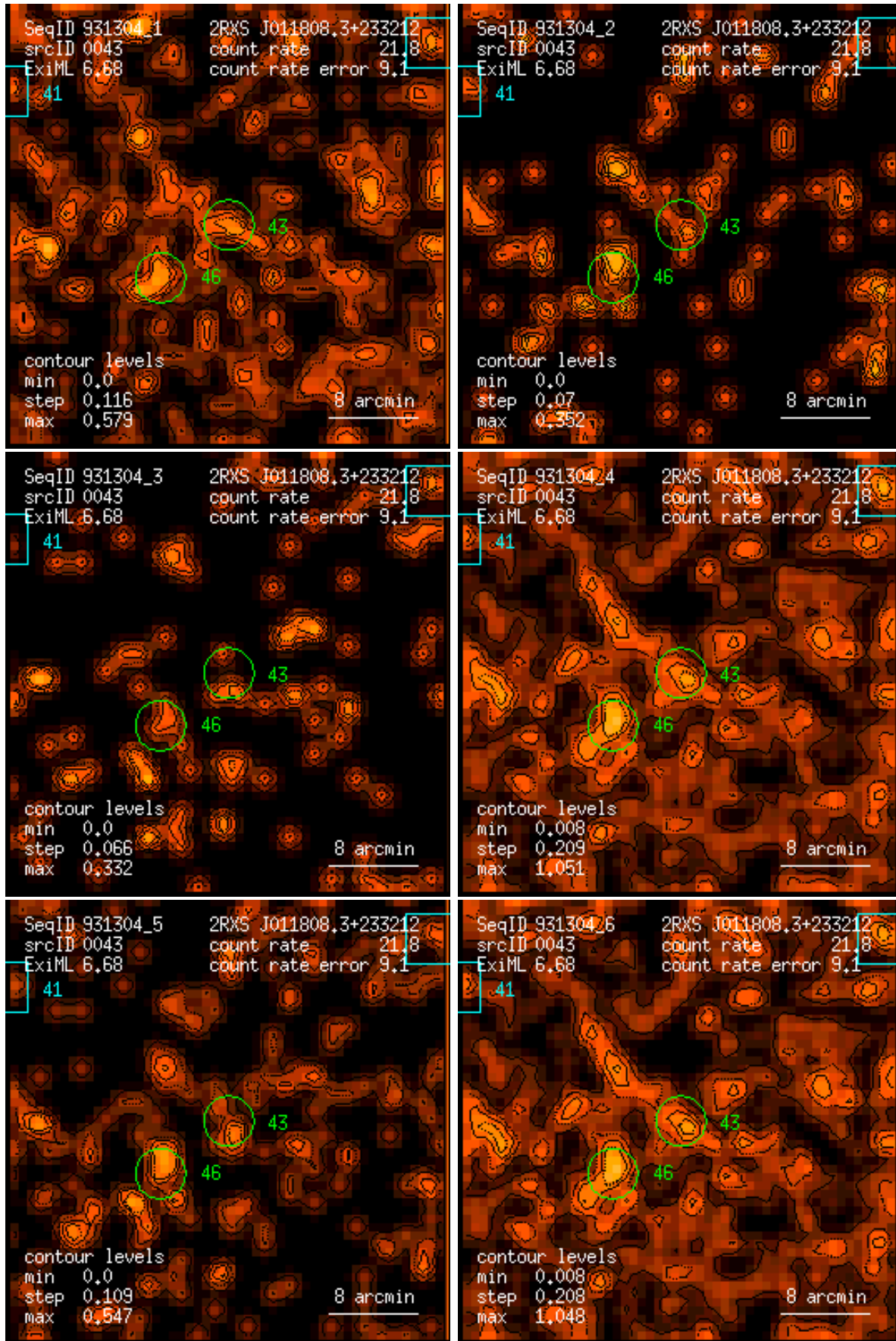
Figure 43: RASS 931304: detection 0043: band rate images, Gaussian filter: (1) PSPC channels 11 – 41, (2) 52 – 90, (3) 91 – 201, (4) 11 – 235, (5) 52 – 201, (6) 11 – 201. Broad band rates in counts/ks. Band rate contour levels in counts/ks/arcmin 2 .
