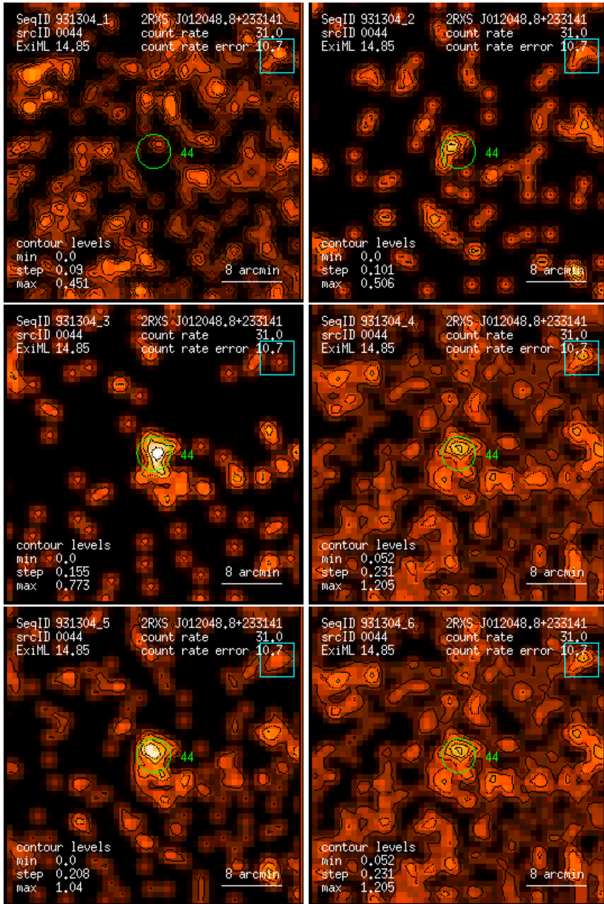
Figure 44: RASS 931304: detection 0044: band rate images, Gaussian filter: (1) PSPC channels 11 – 41, (2) 52 – 90, (3) 91 – 201, (4) 11 – 235, (5) 52 – 201, (6) 11 – 201. Broad band rates in counts/ks. Band rate contour levels in counts/ks/arcmin 2 .
