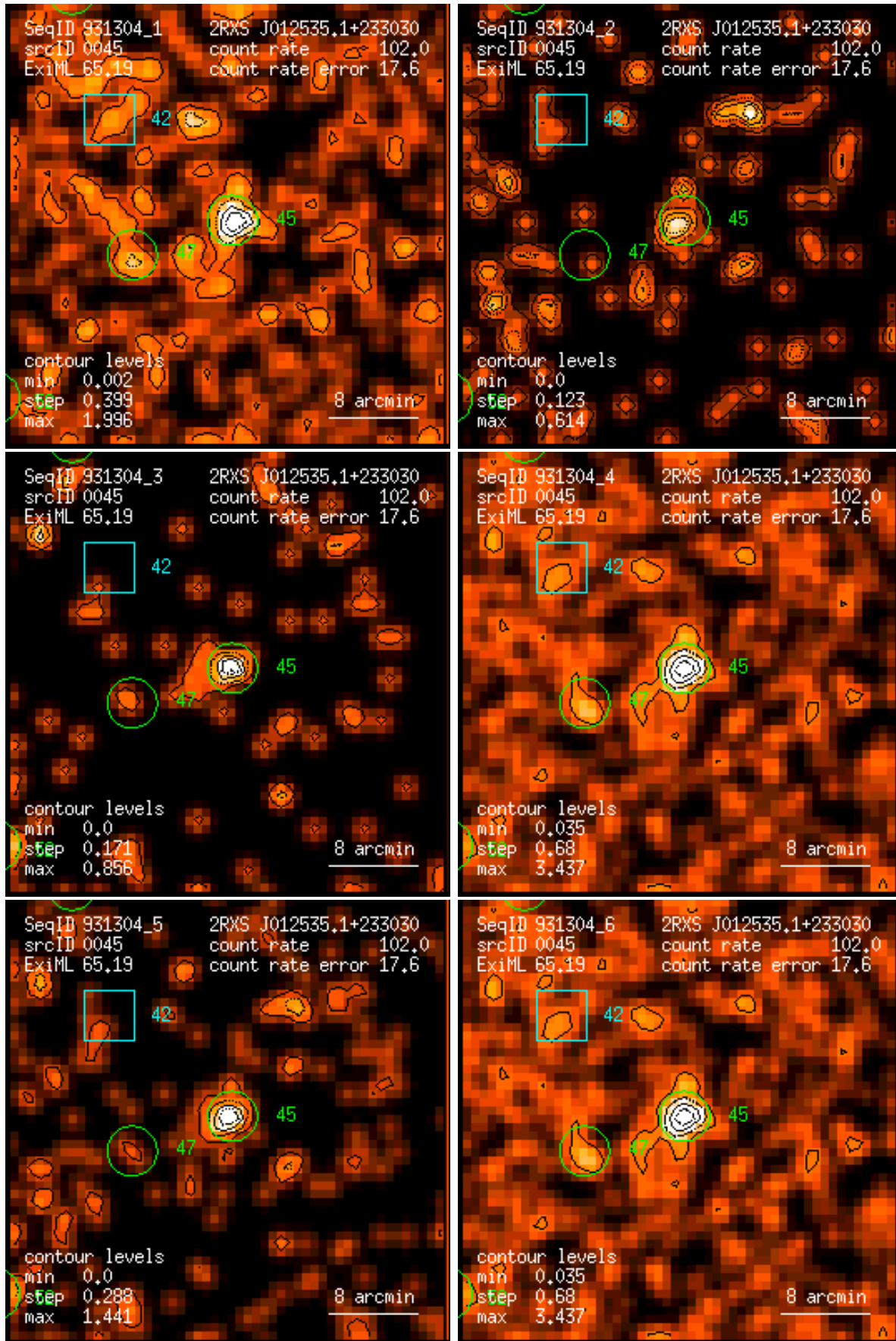
Figure 45: RASS 931304: detection 0045: band rate images, Gaussian filter: (1) PSPC channels 11 – 41, (2) 52 – 90, (3) 91 – 201, (4) 11 – 235, (5) 52 – 201, (6) 11 – 201. Broad band rates in counts/ks. Band rate contour levels in counts/ks/arcmin 2 .
