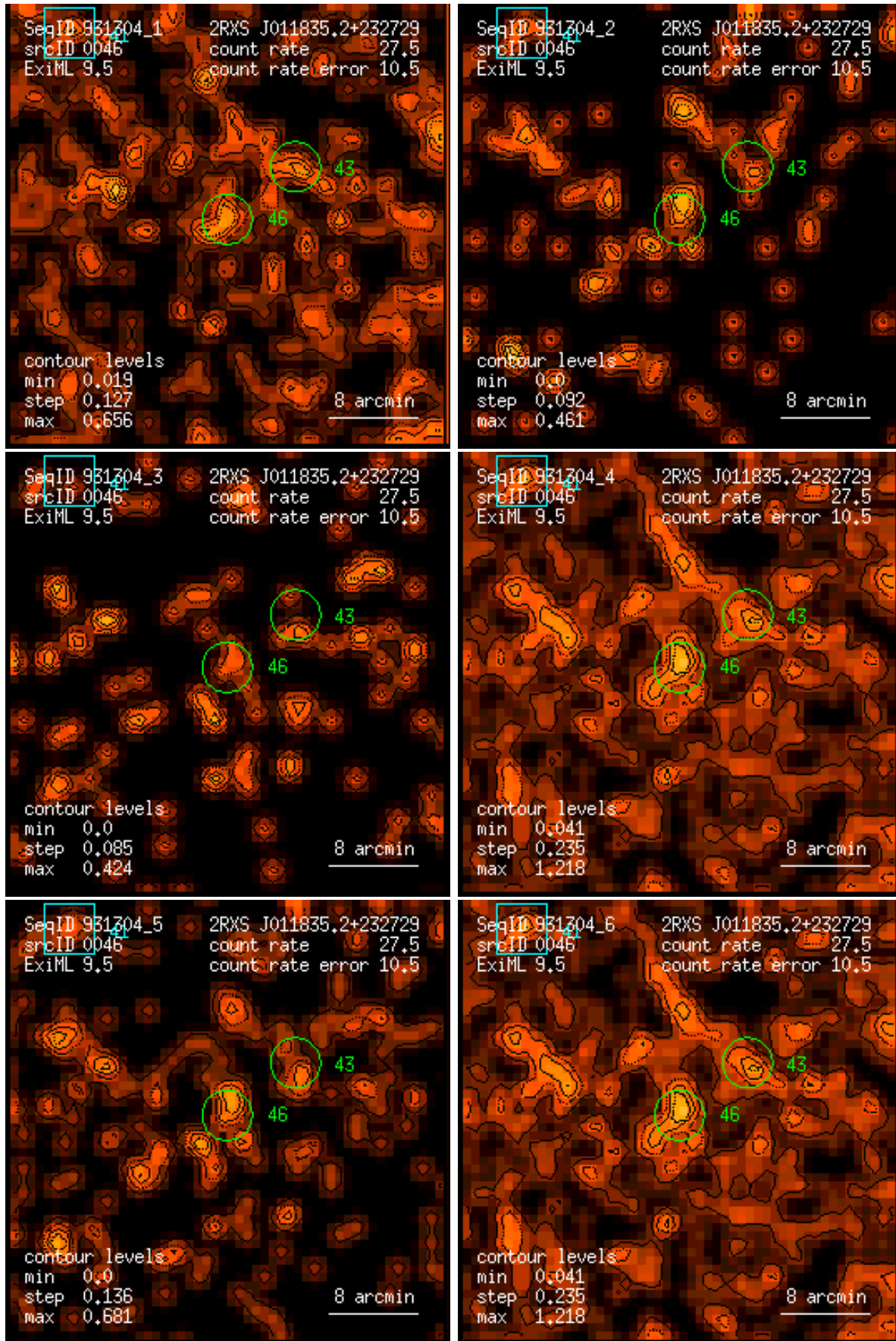
Figure 46: RASS 931304: detection 0046: band rate images, Gaussian filter: (1) PSPC channels 11 – 41, (2) 52 – 90, (3) 91 – 201, (4) 11 – 235, (5) 52 – 201, (6) 11 – 201. Broad band rates in counts/ks. Band rate contour levels in counts/ks/arcmin 2 .
