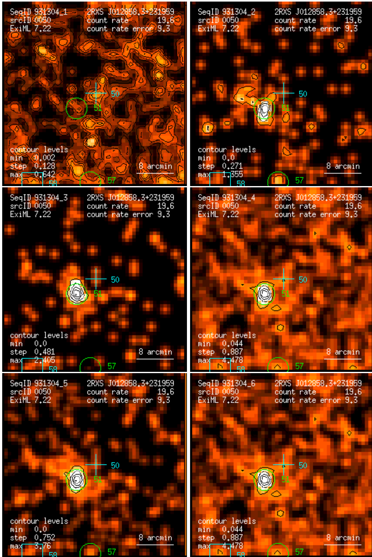
Figure 50: RASS 931304: detection 0050: band rate images, Gaussian filter: (1) PSPC channels 11 – 41, (2) 52 – 90, (3) 91 – 201, (4) 11 – 235, (5) 52 – 201, (6) 11 – 201. Broad band rates in counts/ks. Band rate contour levels in counts/ks/arcmin 2 .
