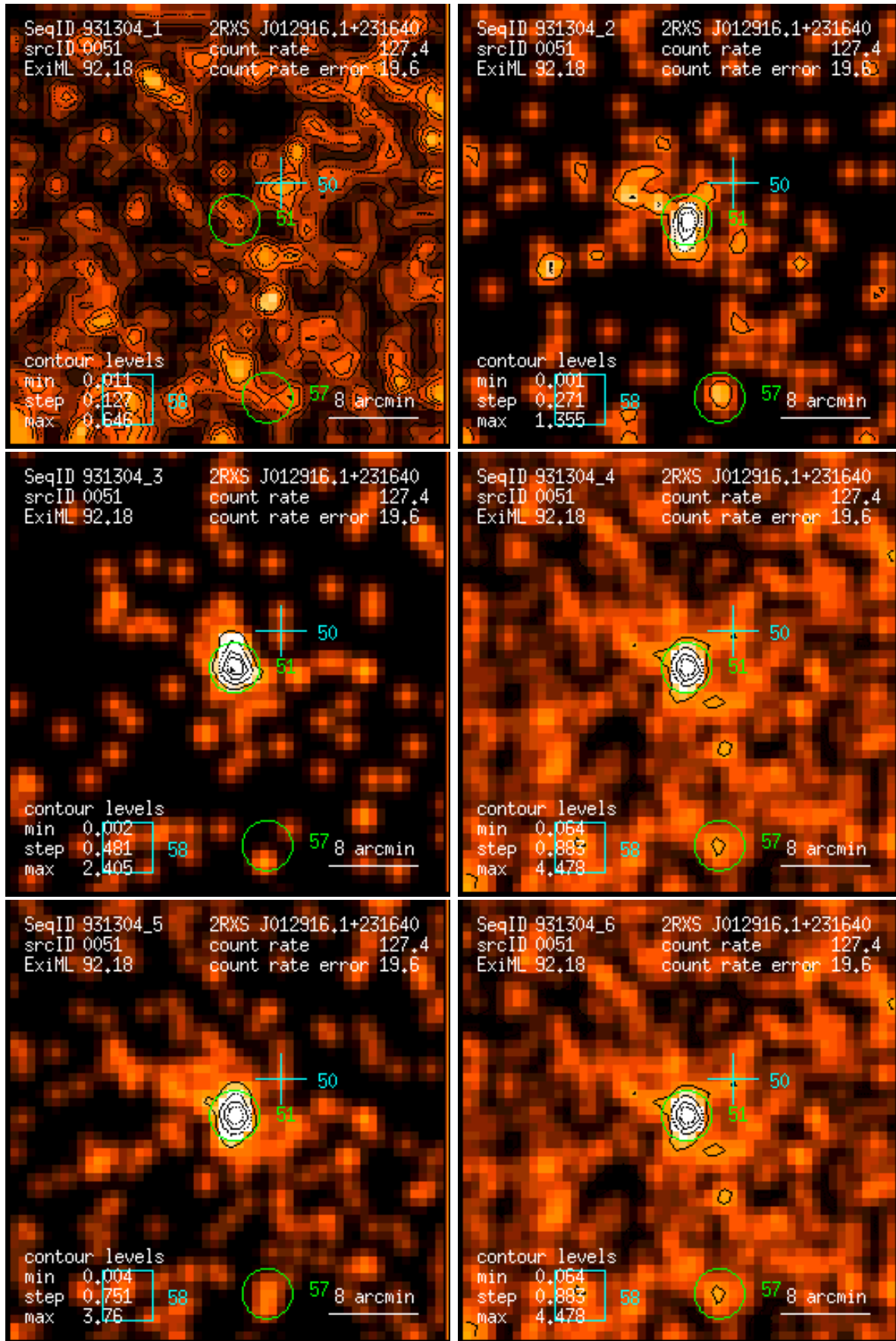
Figure 51: RASS 931304: detection 0051: band rate images, Gaussian filter: (1) PSPC channels 11 – 41, (2) 52 – 90, (3) 91 – 201, (4) 11 – 235, (5) 52 – 201, (6) 11 – 201. Broad band rates in counts/ks. Band rate contour levels in counts/ks/arcmin 2 .
