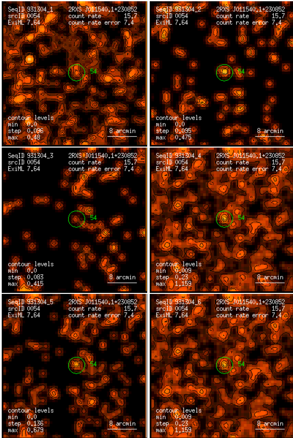
Figure 54: RASS 931304: detection 0054: band rate images, Gaussian filter: (1) PSPC channels 11 – 41, (2) 52 – 90, (3) 91 – 201, (4) 11 – 235, (5) 52 – 201, (6) 11 – 201. Broad band rates in counts/ks. Band rate contour levels in counts/ks/arcmin 2 .
