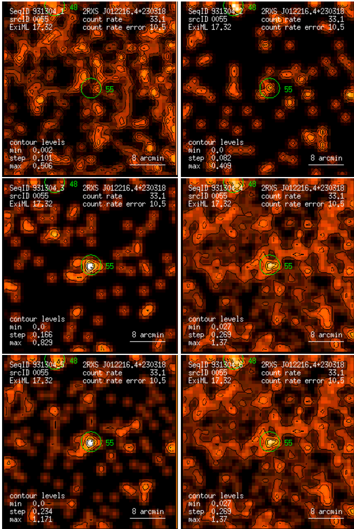
Figure 55: RASS 931304: detection 0055: band rate images, Gaussian filter: (1) PSPC channels 11 – 41, (2) 52 – 90, (3) 91 – 201, (4) 11 – 235, (5) 52 – 201, (6) 11 – 201. Broad band rates in counts/ks. Band rate contour levels in counts/ks/arcmin 2 .
