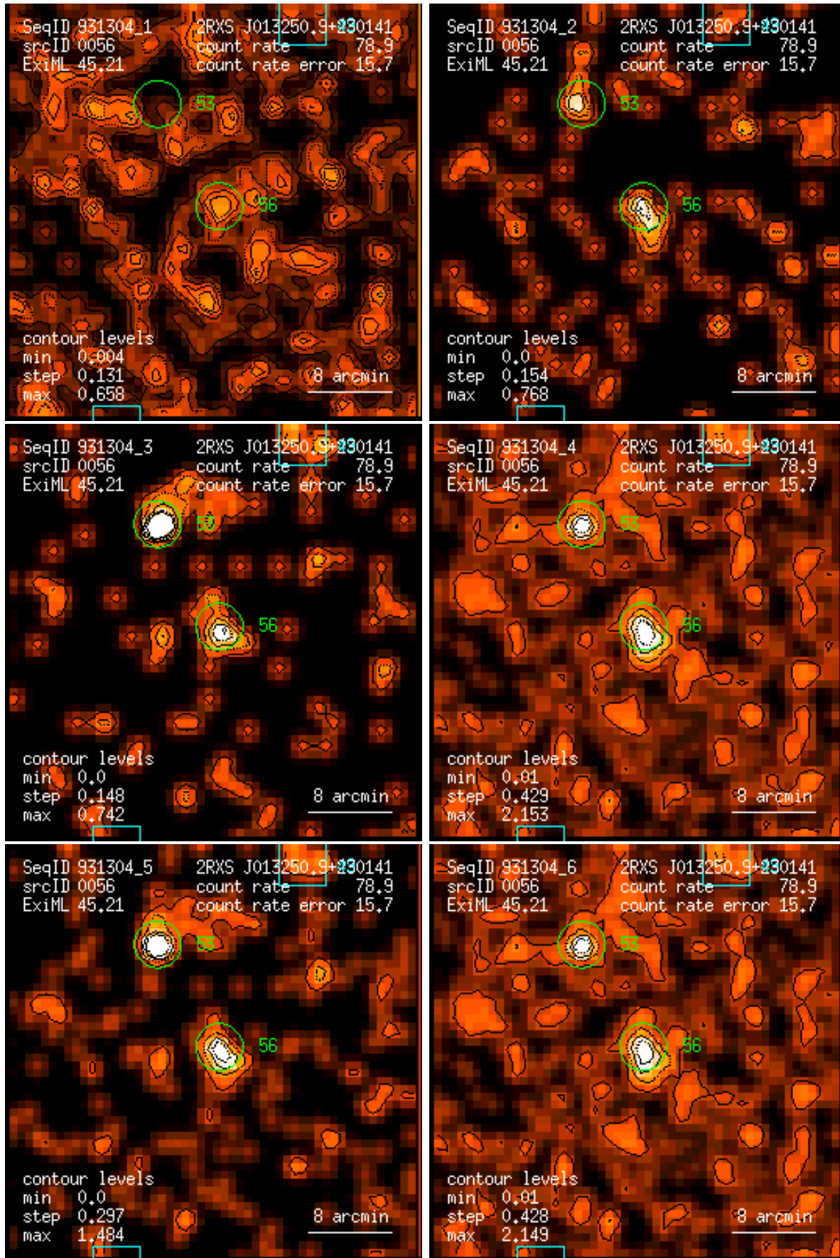
Figure 56: RASS 931304: detection 0056: band rate images, Gaussian filter: (1) PSPC channels 11 – 41, (2) 52 – 90, (3) 91 – 201, (4) 11 – 235, (5) 52 – 201, (6) 11 – 201. Broad band rates in counts/ks. Band rate contour levels in counts/ks/arcmin 2 .
