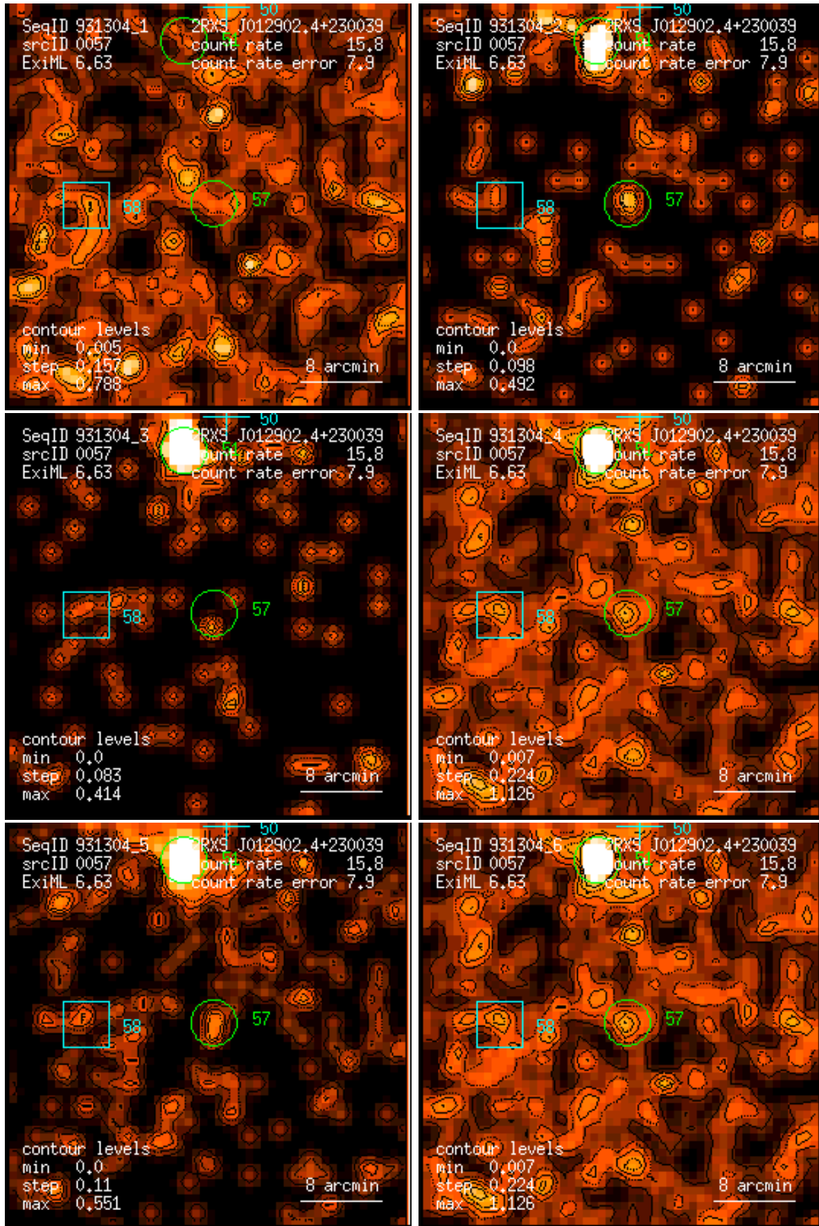
Figure 57: RASS 931304: detection 0057: band rate images, Gaussian filter: (1) PSPC channels 11 – 41, (2) 52 – 90, (3) 91 – 201, (4) 11 – 235, (5) 52 – 201, (6) 11 – 201. Broad band rates in counts/ks. Band rate contour levels in counts/ks/arcmin 2 .
