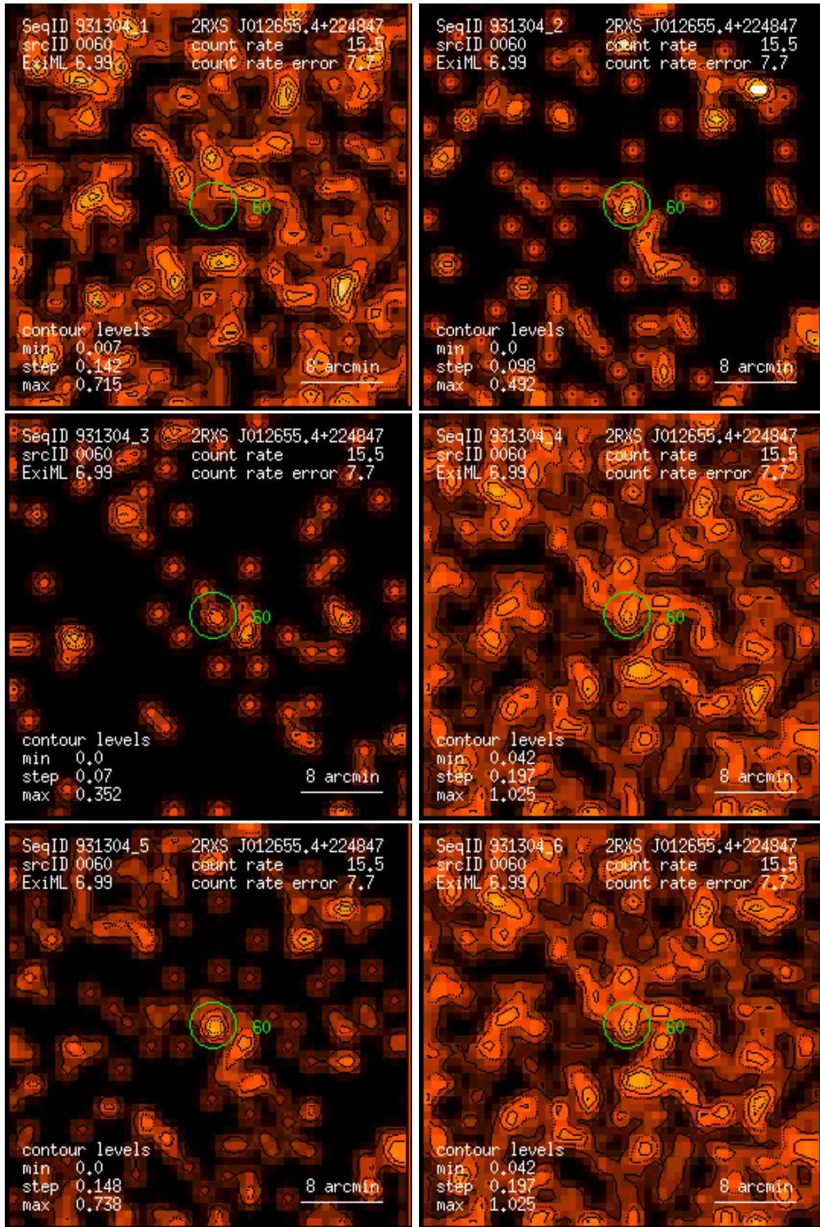
Figure 60: RASS 931304: detection 0060: band rate images, Gaussian filter: (1) PSPC channels 11 – 41, (2) 52 – 90, (3) 91 – 201, (4) 11 – 235, (5) 52 – 201, (6) 11 – 201. Broad band rates in counts/ks. Band rate contour levels in counts/ks/arcmin 2 .
