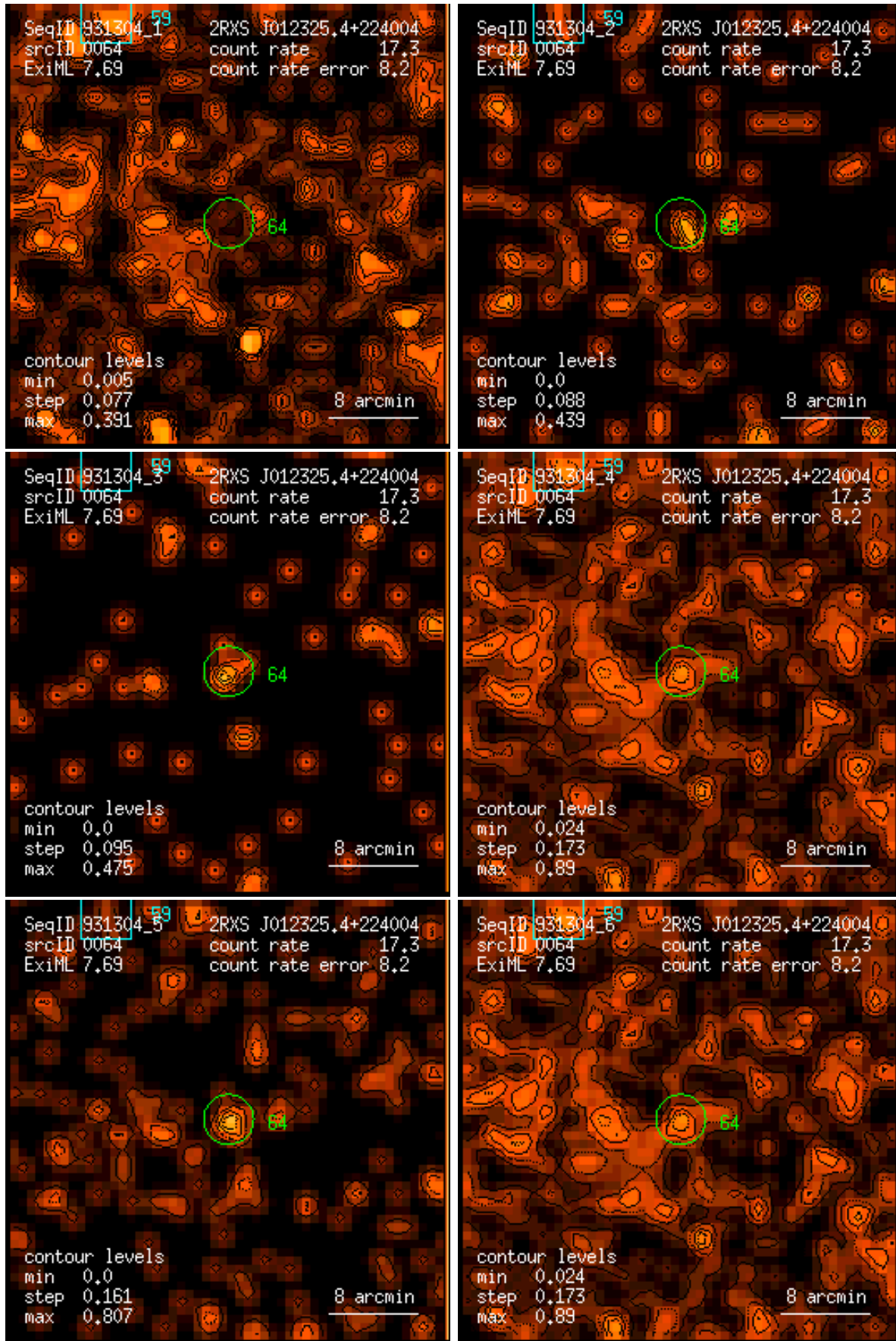
Figure 64: RASS 931304: detection 0064: band rate images, Gaussian filter: (1) PSPC channels 11 – 41, (2) 52 – 90, (3) 91 – 201, (4) 11 – 235, (5) 52 – 201, (6) 11 – 201. Broad band rates in counts/ks. Band rate contour levels in counts/ks/arcmin 2 .
