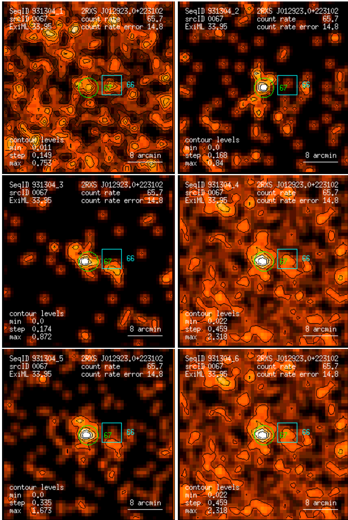
Figure 67: RASS 931304: detection 0067: band rate images, Gaussian filter: (1) PSPC channels 11 – 41, (2) 52 – 90, (3) 91 – 201, (4) 11 – 235, (5) 52 – 201, (6) 11 – 201. Broad band rates in counts/ks. Band rate contour levels in counts/ks/arcmin 2 .
