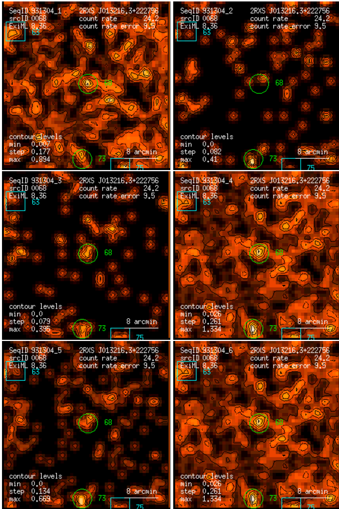
Figure 68: RASS 931304: detection 0068: band rate images, Gaussian filter: (1) PSPC channels 11 – 41, (2) 52 – 90, (3) 91 – 201, (4) 11 – 235, (5) 52 – 201, (6) 11 – 201. Broad band rates in counts/ks. Band rate contour levels in counts/ks/arcmin 2 .
