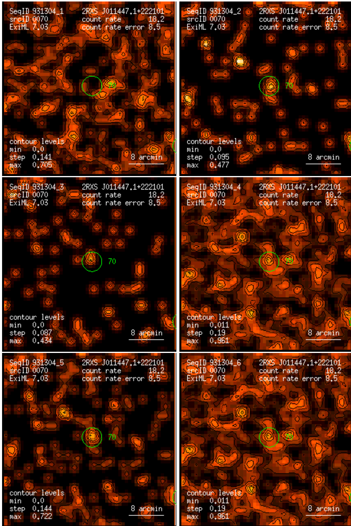
Figure 70: RASS 931304: detection 0070: band rate images, Gaussian filter: (1) PSPC channels 11 – 41, (2) 52 – 90, (3) 91 – 201, (4) 11 – 235, (5) 52 – 201, (6) 11 – 201. Broad band rates in counts/ks. Band rate contour levels in counts/ks/arcmin 2 .
