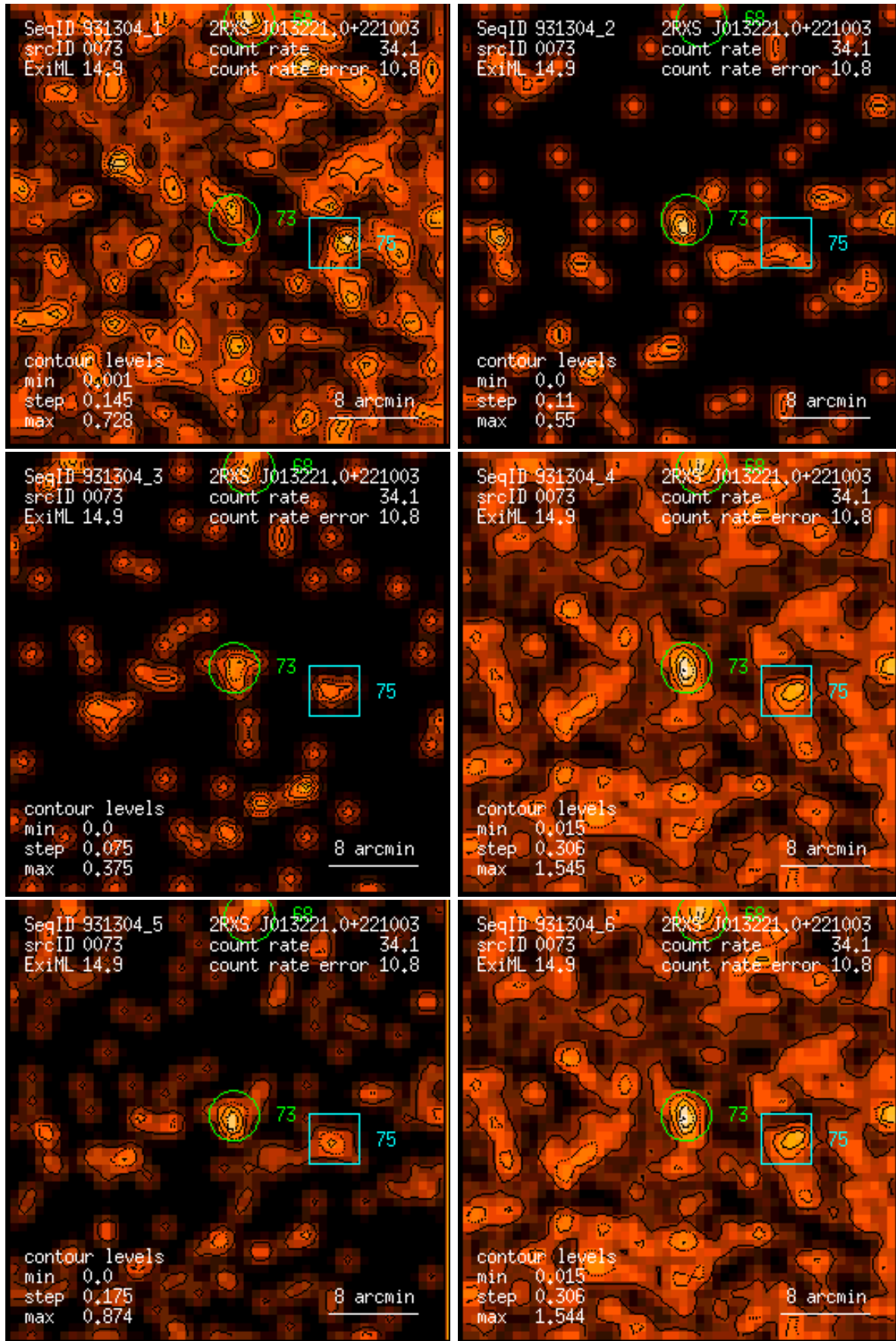
Figure 73: RASS 931304: detection 0073: band rate images, Gaussian filter: (1) PSPC channels 11 – 41, (2) 52 – 90, (3) 91 – 201, (4) 11 – 235, (5) 52 – 201, (6) 11 – 201. Broad band rates in counts/ks. Band rate contour levels in counts/ks/arcmin 2 .
