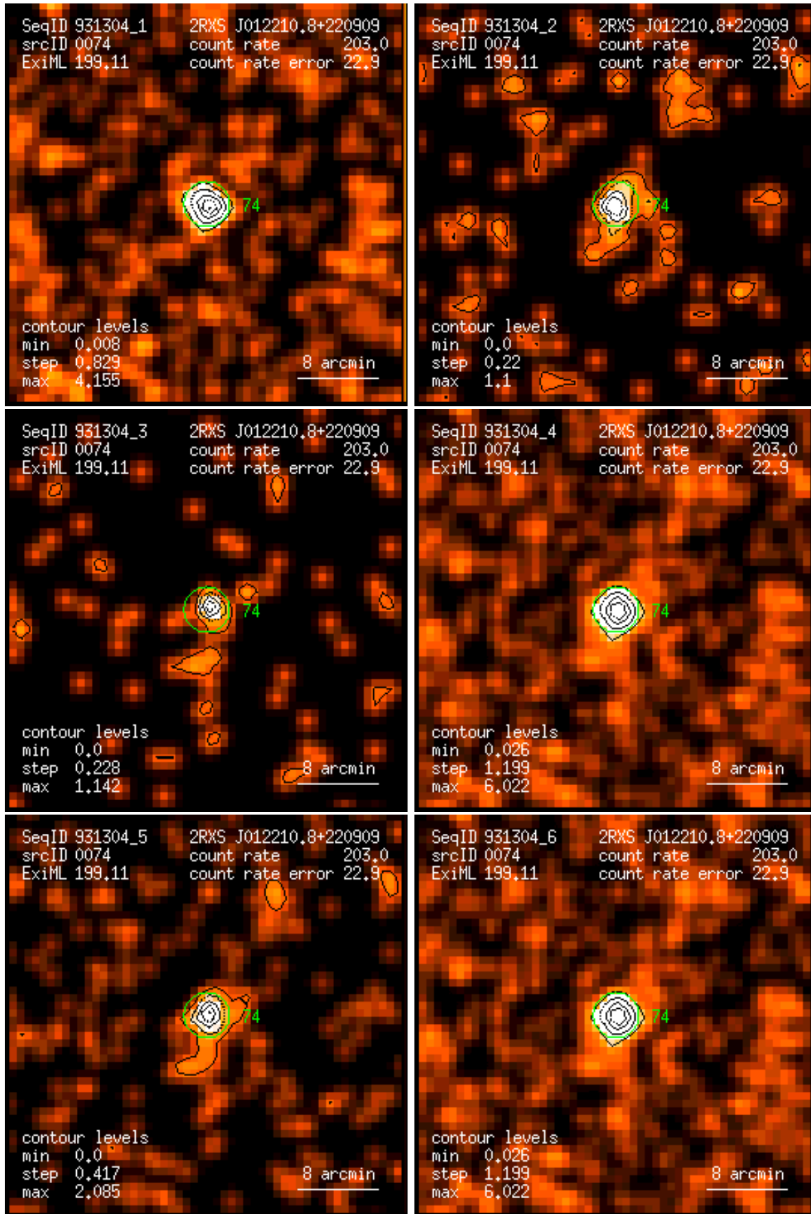
Figure 74: RASS 931304: detection 0074: band rate images, Gaussian filter: (1) PSPC channels 11 – 41, (2) 52 – 90, (3) 91 – 201, (4) 11 – 235, (5) 52 – 201, (6) 11 – 201. Broad band rates in counts/ks. Band rate contour levels in counts/ks/arcmin 2 .
