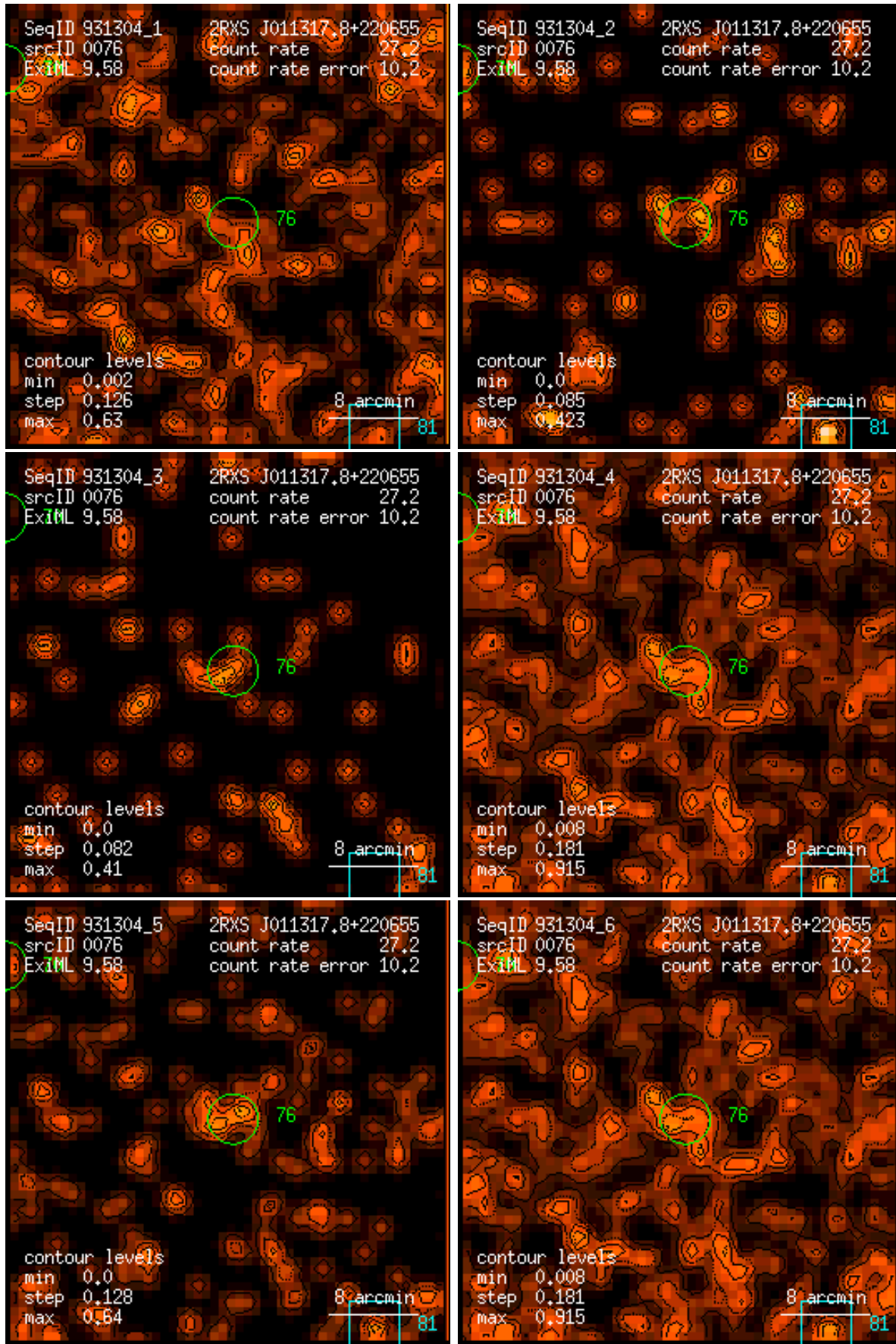
Figure 76: RASS 931304: detection 0076: band rate images, Gaussian filter: (1) PSPC channels 11 – 41, (2) 52 – 90, (3) 91 – 201, (4) 11 – 235, (5) 52 – 201, (6) 11 – 201. Broad band rates in counts/ks. Band rate contour levels in counts/ks/arcmin 2 .
