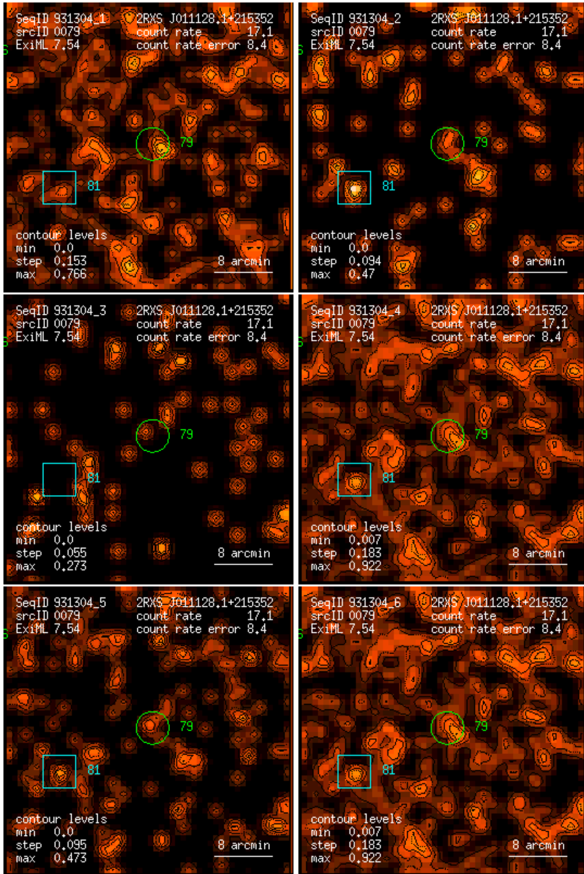
Figure 79: RASS 931304: detection 0079: band rate images, Gaussian filter: (1) PSPC channels 11 – 41, (2) 52 – 90, (3) 91 – 201, (4) 11 – 235, (5) 52 – 201, (6) 11 – 201. Broad band rates in counts/ks. Band rate contour levels in counts/ks/arcmin 2 .
