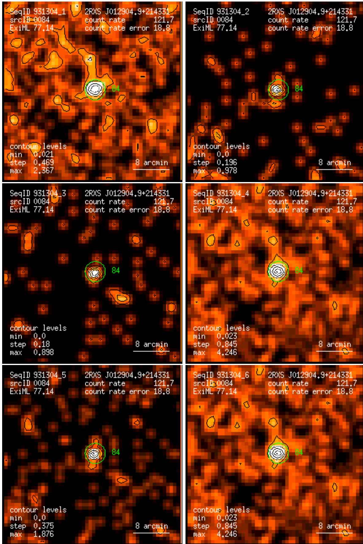
Figure 84: RASS 931304: detection 0084: band rate images, Gaussian filter: (1) PSPC channels 11 – 41, (2) 52 – 90, (3) 91 – 201, (4) 11 – 235, (5) 52 – 201, (6) 11 – 201. Broad band rates in counts/ks. Band rate contour levels in counts/ks/arcmin 2 .
