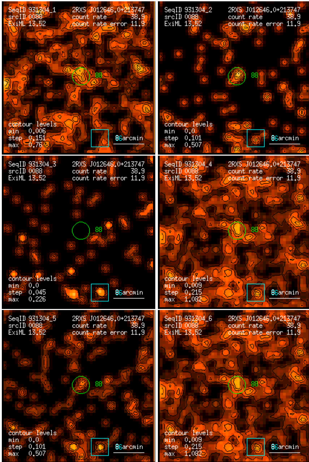
Figure 88: RASS 931304: detection 0088: band rate images, Gaussian filter: (1) PSPC channels 11 – 41, (2) 52 – 90, (3) 91 – 201, (4) 11 – 235, (5) 52 – 201, (6) 11 – 201. Broad band rates in counts/ks. Band rate contour levels in counts/ks/arcmin 2 .
