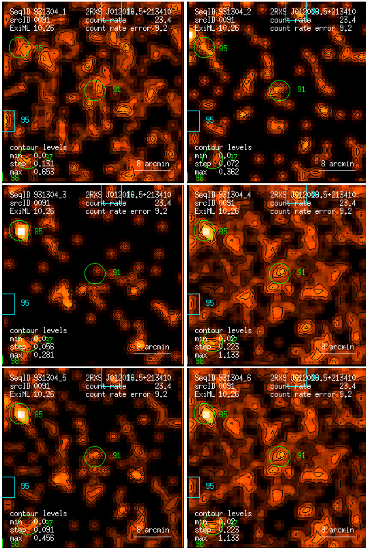
Figure 91: RASS 931304: detection 0091: band rate images, Gaussian filter: (1) PSPC channels 11 – 41, (2) 52 – 90, (3) 91 – 201, (4) 11 – 235, (5) 52 – 201, (6) 11 – 201. Broad band rates in counts/ks. Band rate contour levels in counts/ks/arcmin 2 .
