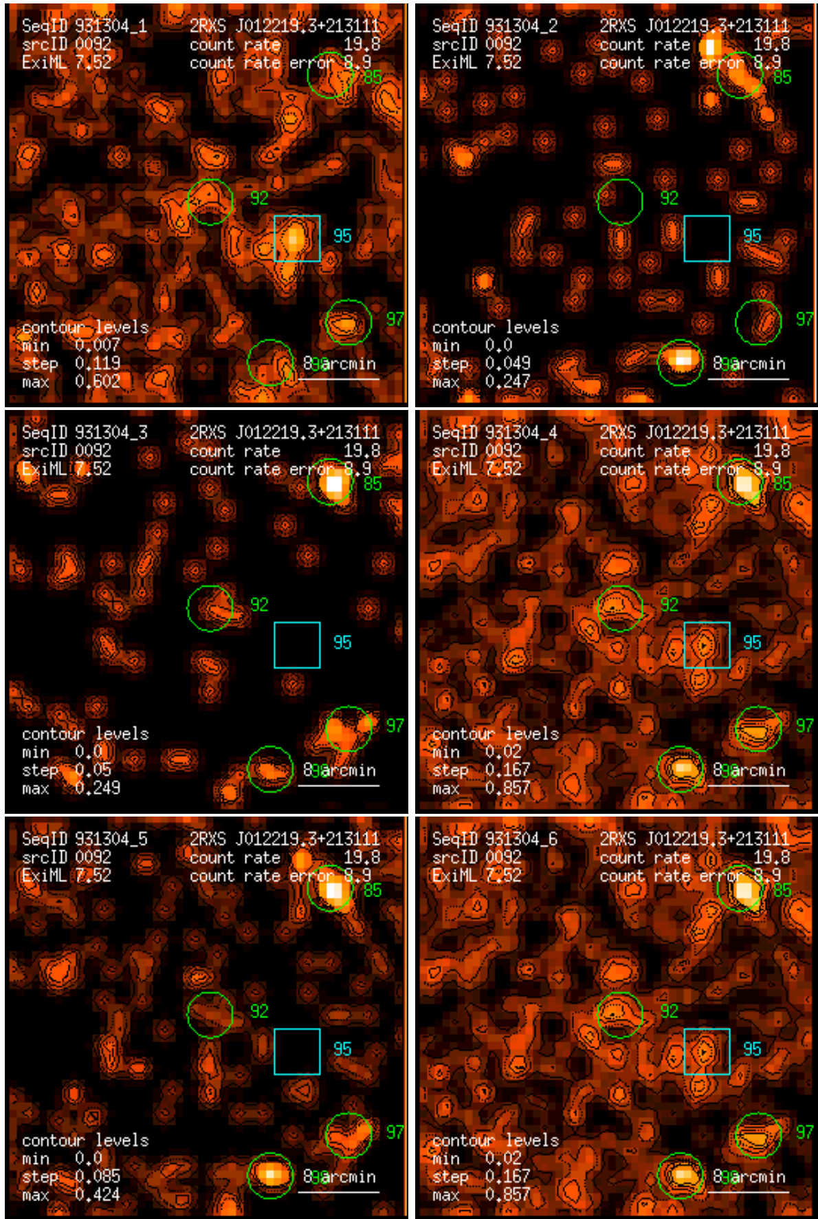
Figure 92: RASS 931304: detection 0092: band rate images, Gaussian filter: (1) PSPC channels 11 – 41, (2) 52 – 90, (3) 91 – 201, (4) 11 – 235, (5) 52 – 201, (6) 11 – 201. Broad band rates in counts/ks. Band rate contour levels in counts/ks/arcmin 2 .
