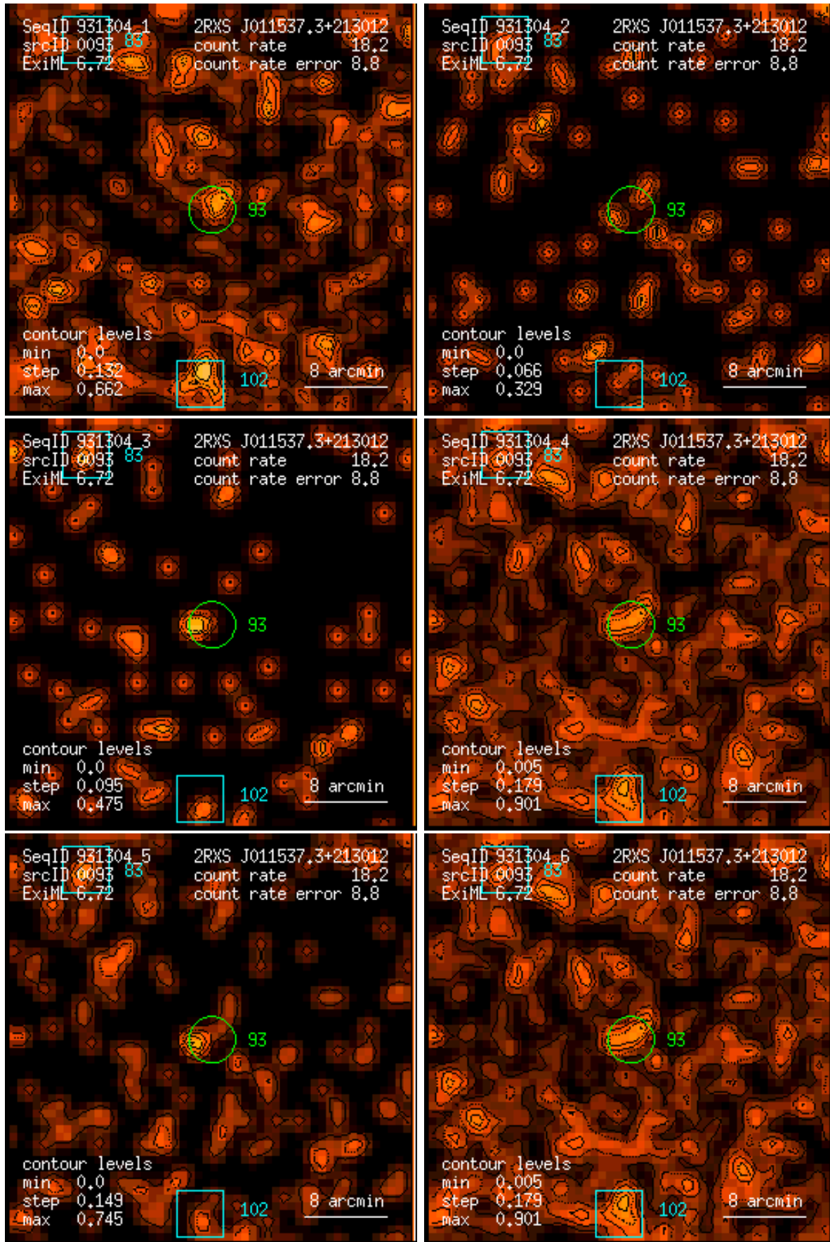
Figure 93: RASS 931304: detection 0093: band rate images, Gaussian filter: (1) PSPC channels 11 – 41, (2) 52 – 90, (3) 91 – 201, (4) 11 – 235, (5) 52 – 201, (6) 11 – 201. Broad band rates in counts/ks. Band rate contour levels in counts/ks/arcmin 2 .
