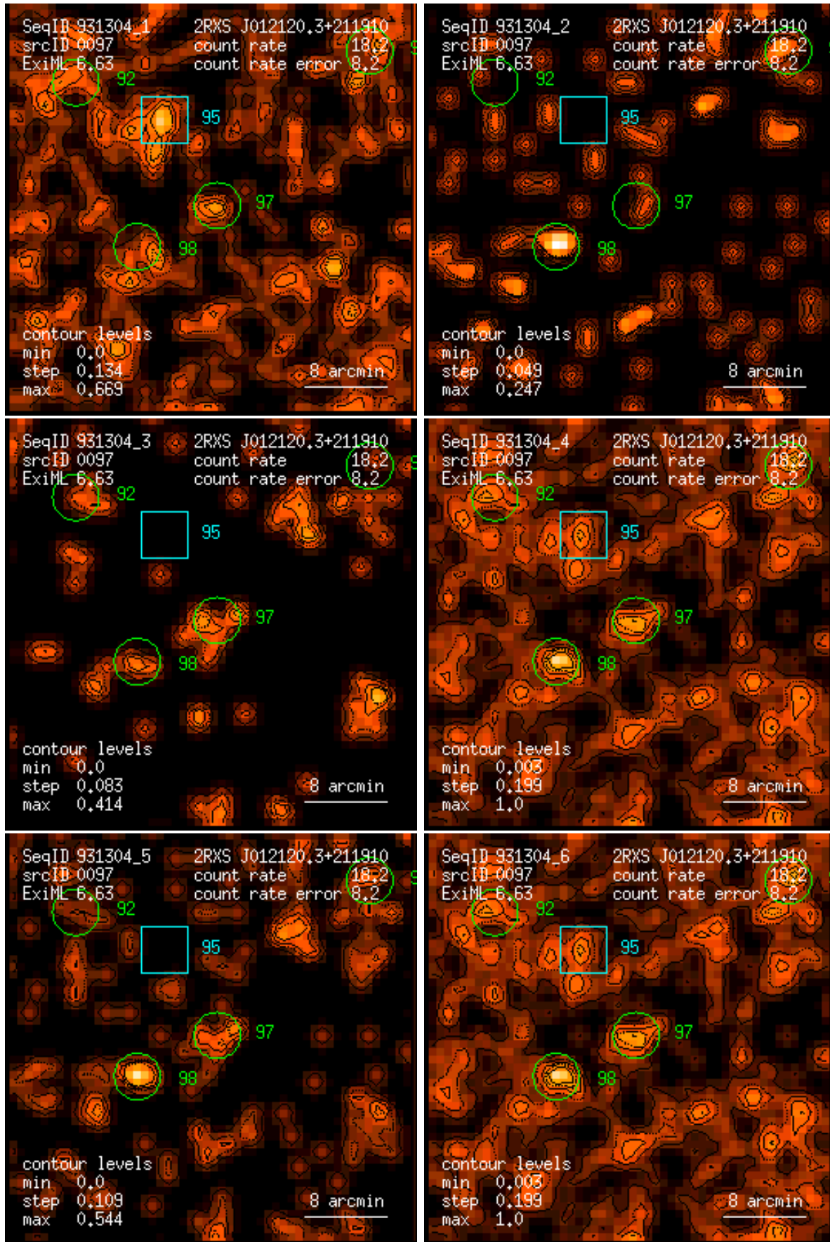
Figure 97: RASS 931304: detection 0097: band rate images, Gaussian filter: (1) PSPC channels 11 – 41, (2) 52 – 90, (3) 91 – 201, (4) 11 – 235, (5) 52 – 201, (6) 11 – 201. Broad band rates in counts/ks. Band rate contour levels in counts/ks/arcmin 2 .
