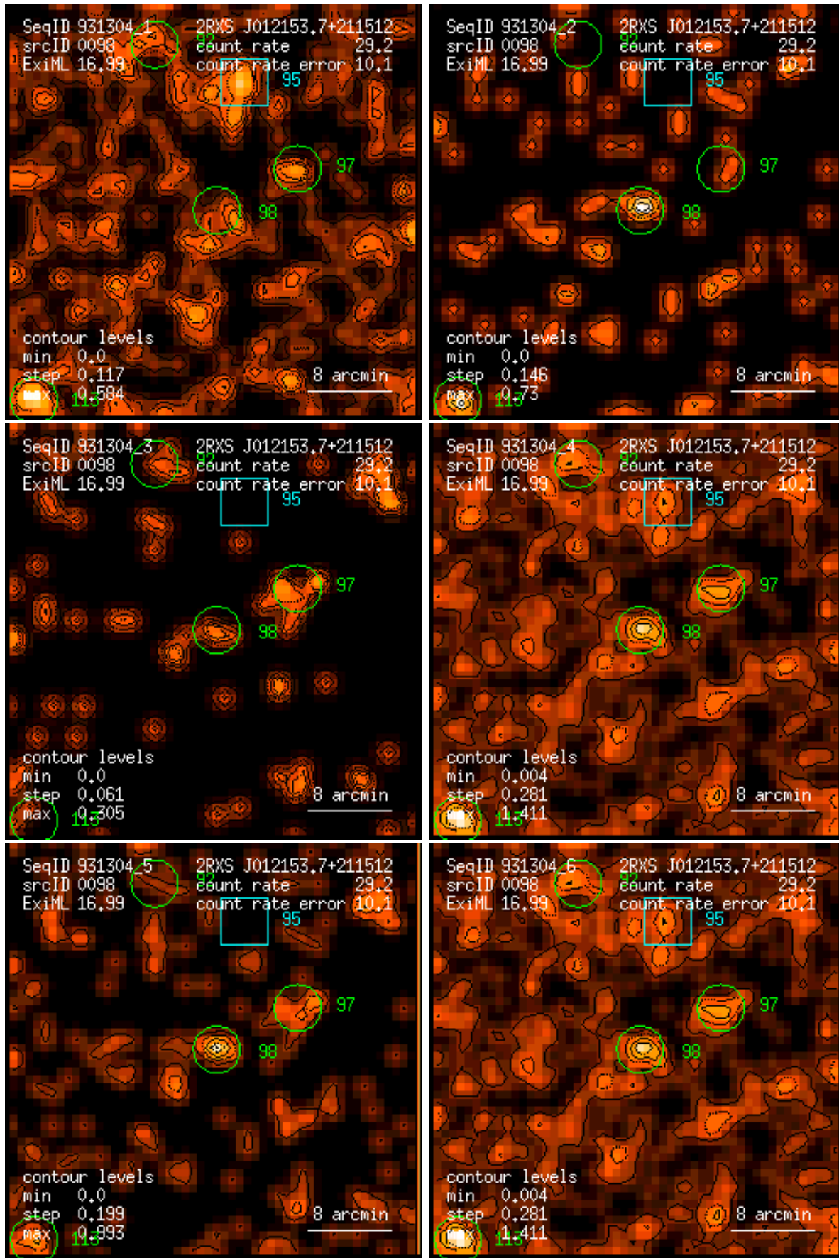
Figure 98: RASS 931304: detection 0098: band rate images, Gaussian filter: (1) PSPC channels 11 – 41, (2) 52 – 90, (3) 91 – 201, (4) 11 – 235, (5) 52 – 201, (6) 11 – 201. Broad band rates in counts/ks. Band rate contour levels in counts/ks/arcmin 2 .
