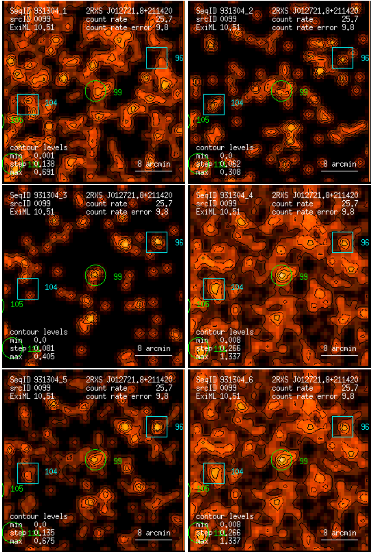
Figure 99: RASS 931304: detection 0099: band rate images, Gaussian filter: (1) PSPC channels 11 – 41, (2) 52 – 90, (3) 91 – 201, (4) 11 – 235, (5) 52 – 201, (6) 11 – 201. Broad band rates in counts/ks. Band rate contour levels in counts/ks/arcmin 2 .
