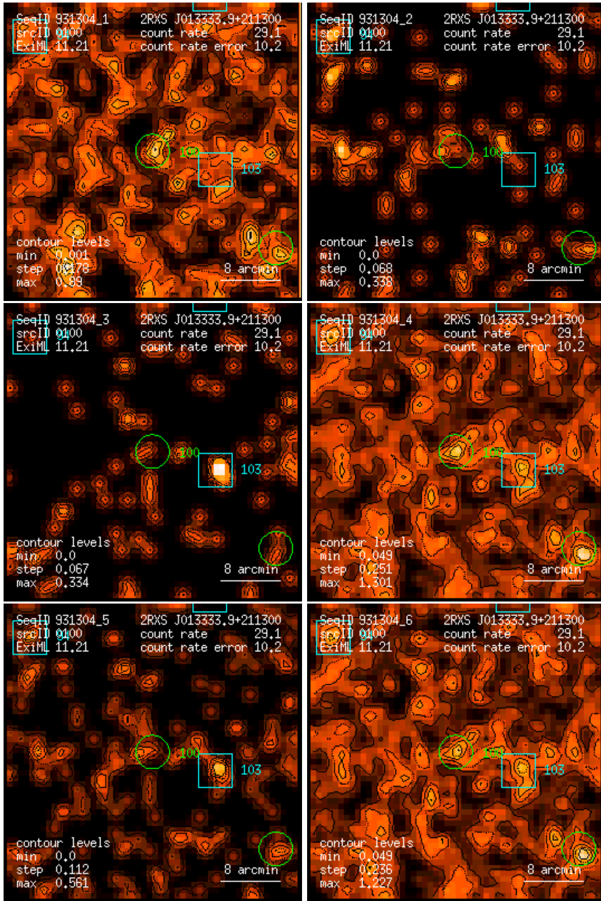
Figure 100: RASS 931304: detection 0100: band rate images, Gaussian filter: (1) PSPC channels 11 – 41, (2) 52 – 90, (3) 91 – 201, (4) 11 – 235, (5) 52 – 201, (6) 11 – 201. Broad band rates in counts/ks. Band rate contour levels in counts/ks/arcmin 2 .
