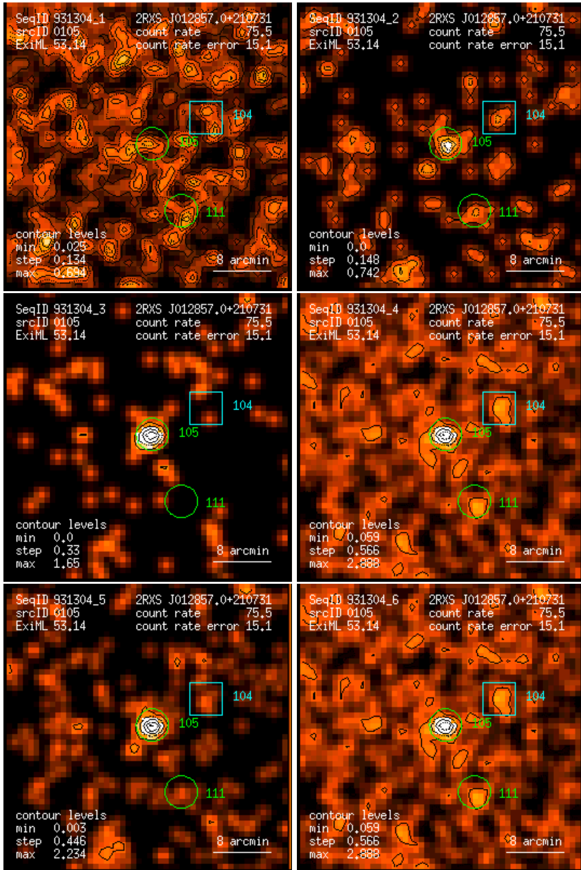
Figure 105: RASS 931304: detection 0105: band rate images, Gaussian filter: (1) PSPC channels 11 – 41, (2) 52 – 90, (3) 91 – 201, (4) 11 – 235, (5) 52 – 201, (6) 11 – 201. Broad band rates in counts/ks. Band rate contour levels in counts/ks/arcmin 2 .
