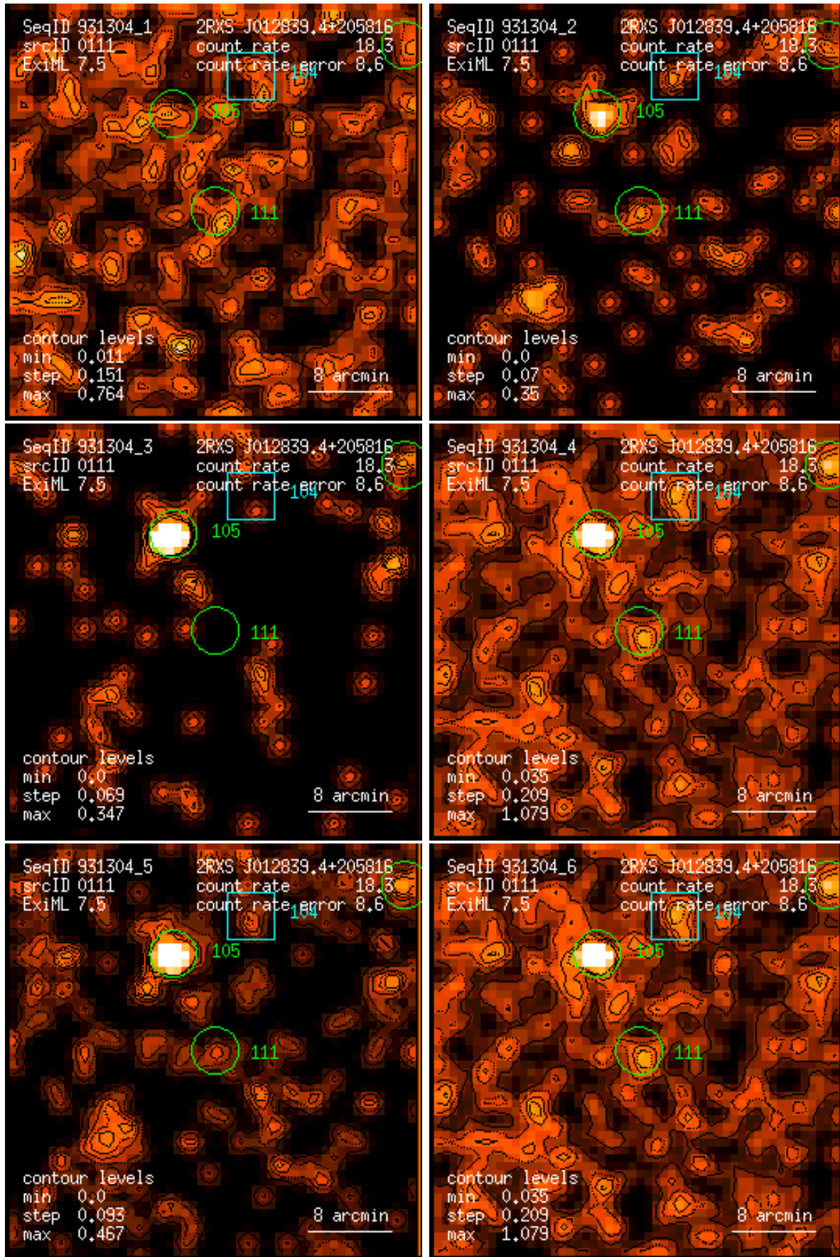
Figure 111: RASS 931304: detection 0111: band rate images, Gaussian filter: (1) PSPC channels 11 – 41, (2) 52 – 90, (3) 91 – 201, (4) 11 – 235, (5) 52 – 201, (6) 11 – 201. Broad band rates in counts/ks. Band rate contour levels in counts/ks/arcmin 2 .
