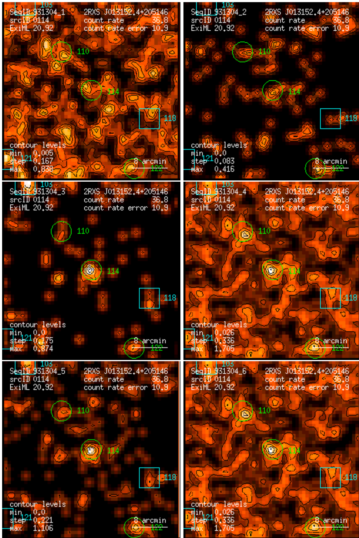
Figure 114: RASS 931304: detection 0114: band rate images, Gaussian filter: (1) PSPC channels 11 – 41, (2) 52 – 90, (3) 91 – 201, (4) 11 – 235, (5) 52 – 201, (6) 11 – 201. Broad band rates in counts/ks. Band rate contour levels in counts/ks/arcmin 2 .
