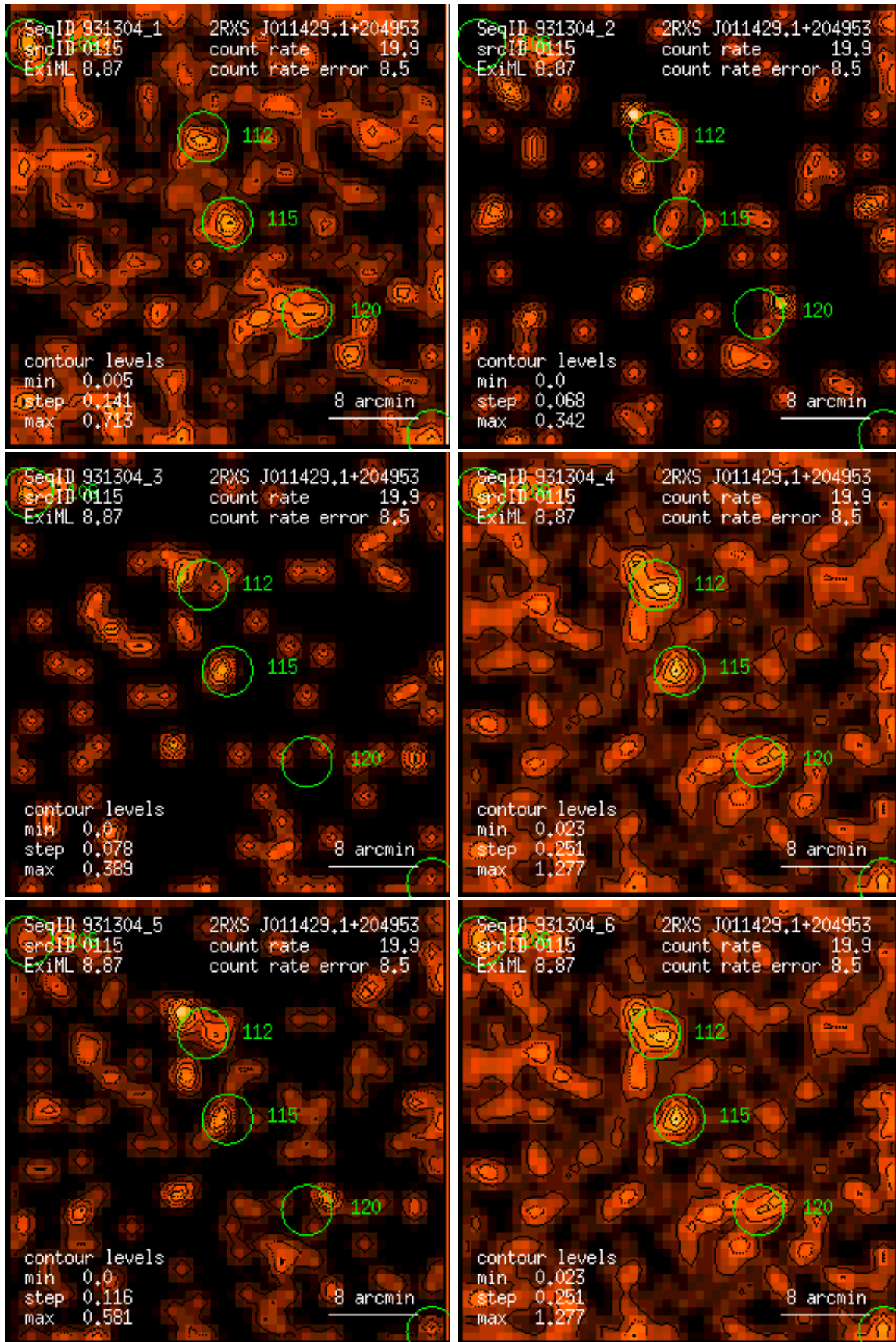
Figure 115: RASS 931304: detection 0115: band rate images, Gaussian filter: (1) PSPC channels 11 – 41, (2) 52 – 90, (3) 91 – 201, (4) 11 – 235, (5) 52 – 201, (6) 11 – 201. Broad band rates in counts/ks. Band rate contour levels in counts/ks/arcmin 2 .
