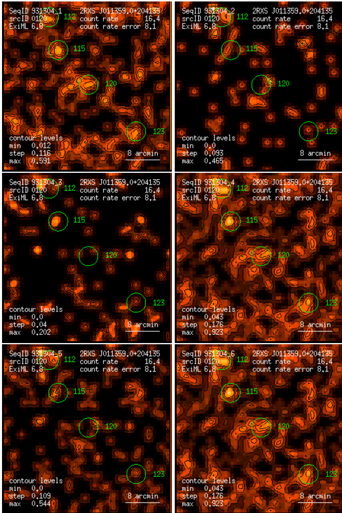
Figure 120: RASS 931304: detection 0120: band rate images, Gaussian filter: (1) PSPC channels 11 – 41, (2) 52 – 90, (3) 91 – 201, (4) 11 – 235, (5) 52 – 201, (6) 11 – 201. Broad band rates in counts/ks. Band rate contour levels in counts/ks/arcmin 2 .
