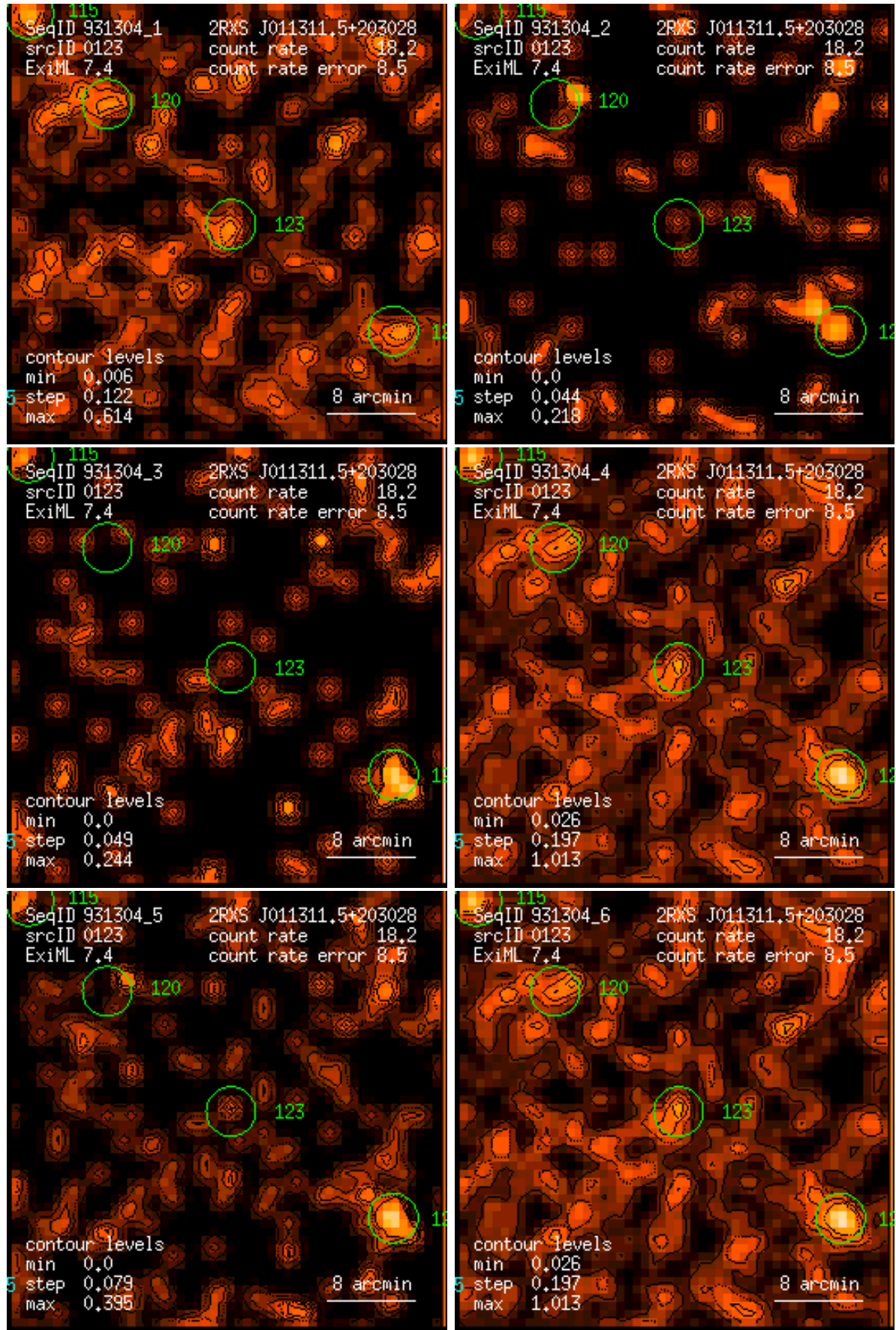
Figure 123: RASS 931304: detection 0123: band rate images, Gaussian filter: (1) PSPC channels 11 – 41, (2) 52 – 90, (3) 91 – 201, (4) 11 – 235, (5) 52 – 201, (6) 11 – 201. Broad band rates in counts/ks. Band rate contour levels in counts/ks/arcmin 2 .
