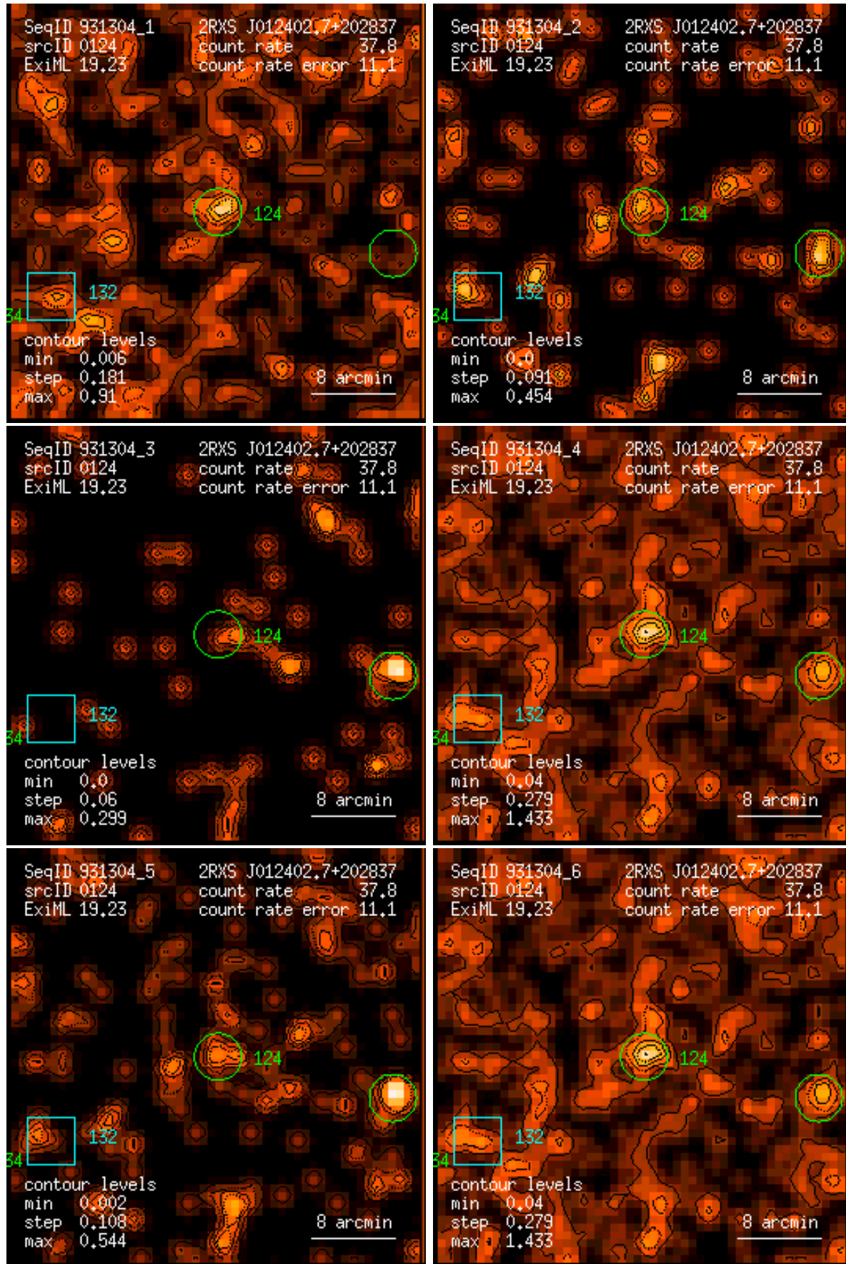
Figure 124: RASS 931304: detection 0124: band rate images, Gaussian filter: (1) PSPC channels 11 – 41, (2) 52 – 90, (3) 91 – 201, (4) 11 – 235, (5) 52 – 201, (6) 11 – 201. Broad band rates in counts/ks. Band rate contour levels in counts/ks/arcmin 2 .
