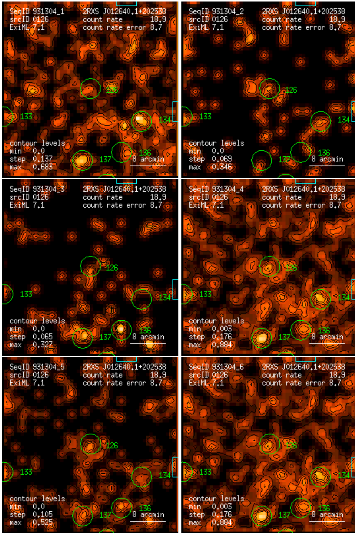
Figure 126: RASS 931304: detection 0126: band rate images, Gaussian filter: (1) PSPC channels 11 – 41, (2) 52 – 90, (3) 91 – 201, (4) 11 – 235, (5) 52 – 201, (6) 11 – 201. Broad band rates in counts/ks. Band rate contour levels in counts/ks/arcmin 2 .
