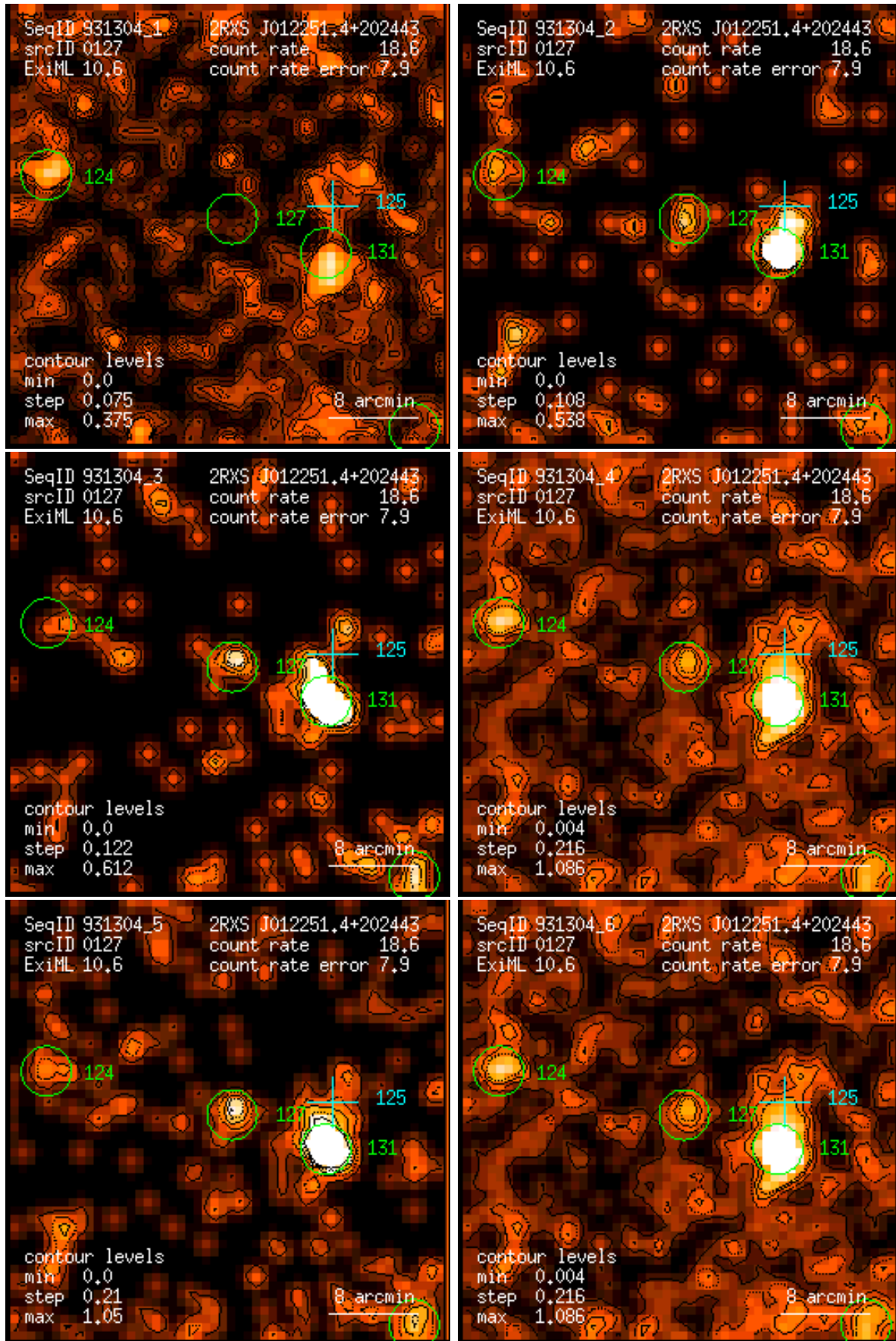
Figure 127: RASS 931304: detection 0127: band rate images, Gaussian filter: (1) PSPC channels 11 – 41, (2) 52 – 90, (3) 91 – 201, (4) 11 – 235, (5) 52 – 201, (6) 11 – 201. Broad band rates in counts/ks. Band rate contour levels in counts/ks/arcmin 2 .
