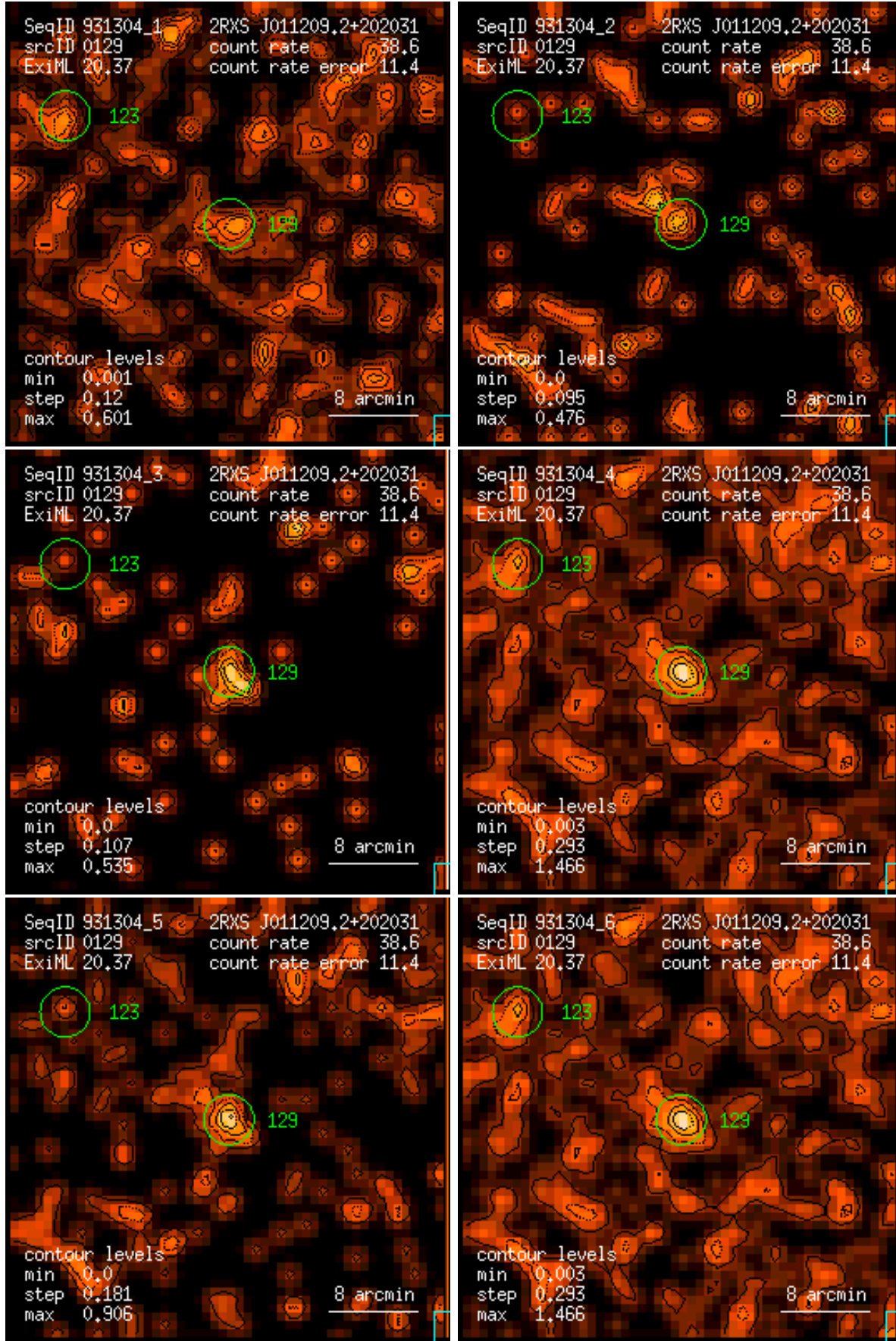
Figure 129: RASS 931304: detection 0129: band rate images, Gaussian filter: (1) PSPC channels 11 – 41, (2) 52 – 90, (3) 91 – 201, (4) 11 – 235, (5) 52 – 201, (6) 11 – 201. Broad band rates in counts/ks. Band rate contour levels in counts/ks/arcmin 2 .
