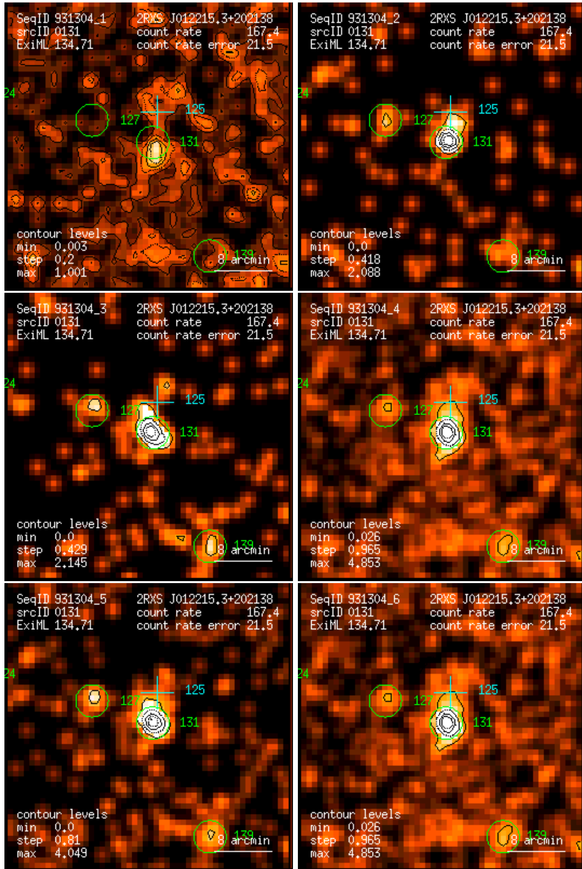
Figure 131: RASS 931304: detection 0131: band rate images, Gaussian filter: (1) PSPC channels 11 – 41, (2) 52 – 90, (3) 91 – 201, (4) 11 – 235, (5) 52 – 201, (6) 11 – 201. Broad band rates in counts/ks. Band rate contour levels in counts/ks/arcmin 2 .
