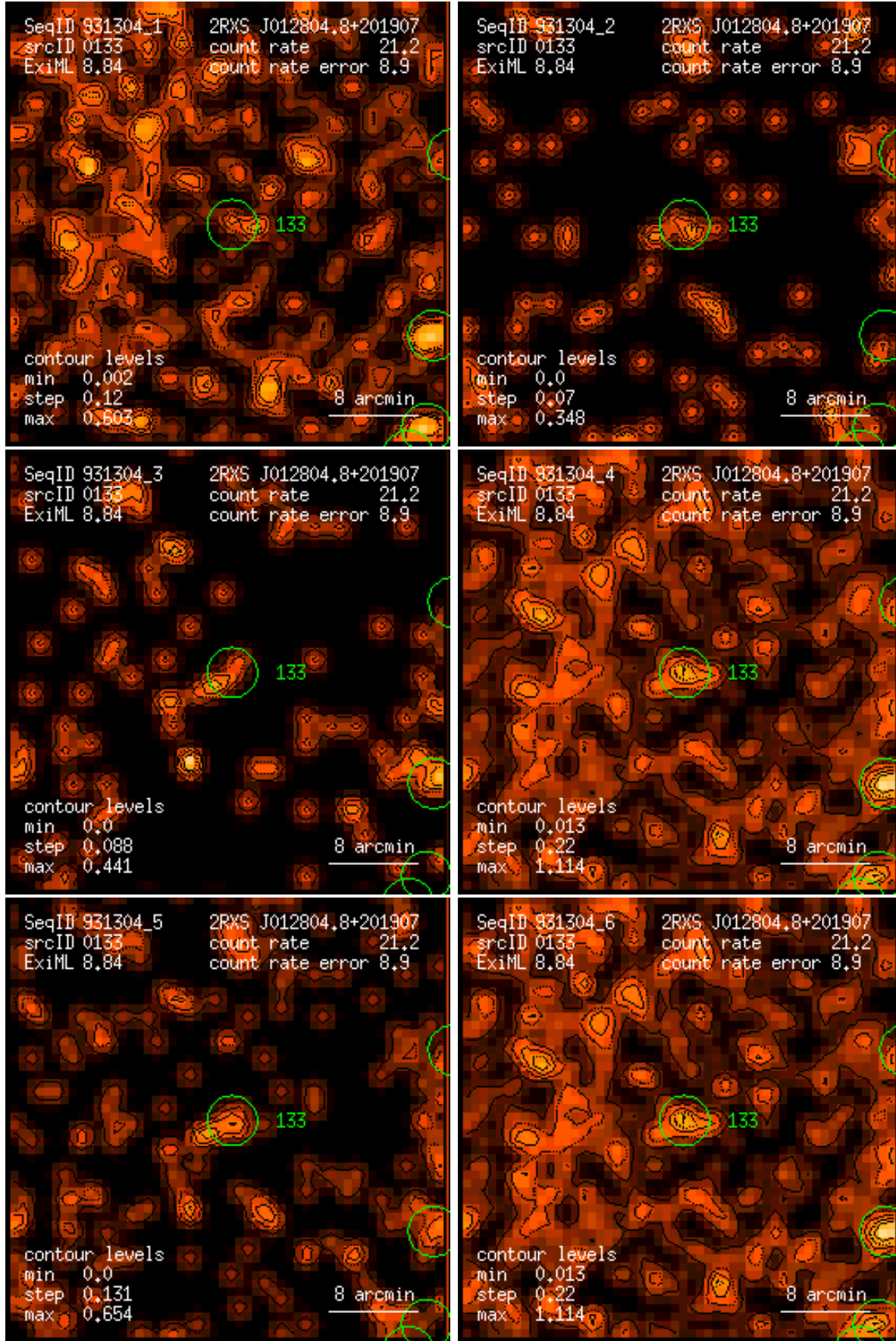
Figure 133: RASS 931304: detection 0133: band rate images, Gaussian filter: (1) PSPC channels 11 – 41, (2) 52 – 90, (3) 91 – 201, (4) 11 – 235, (5) 52 – 201, (6) 11 – 201. Broad band rates in counts/ks. Band rate contour levels in counts/ks/arcmin 2 .
