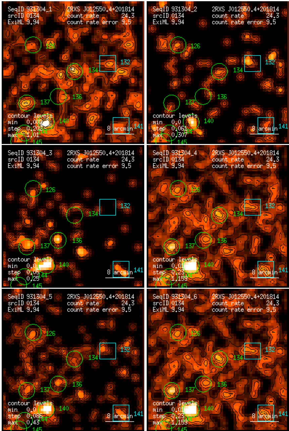
Figure 134: RASS 931304: detection 0134: band rate images, Gaussian filter: (1) PSPC channels 11 – 41, (2) 52 – 90, (3) 91 – 201, (4) 11 – 235, (5) 52 – 201, (6) 11 – 201. Broad band rates in counts/ks. Band rate contour levels in counts/ks/arcmin 2 .
