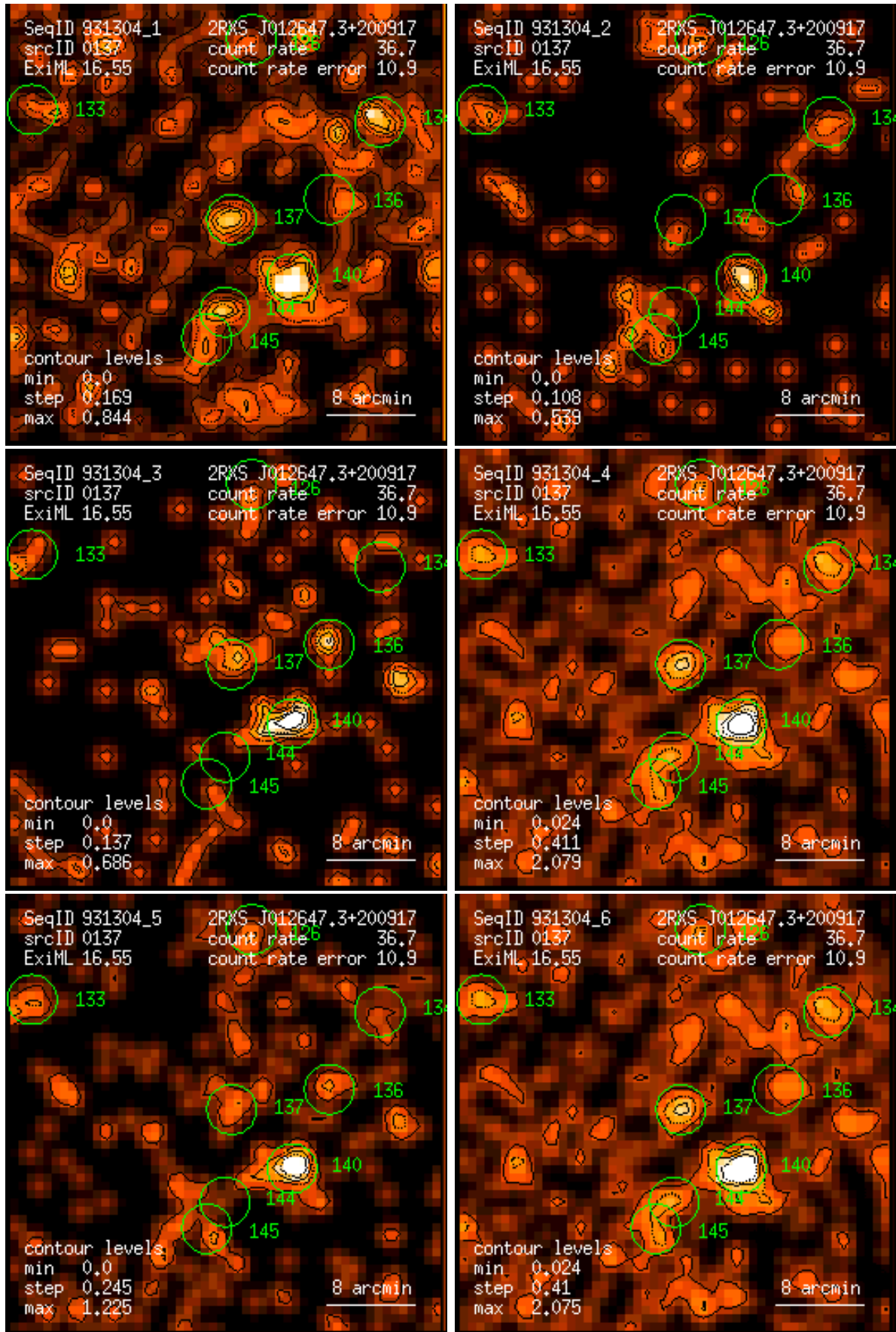
Figure 137: RASS 931304: detection 0137: band rate images, Gaussian filter: (1) PSPC channels 11 – 41, (2) 52 – 90, (3) 91 – 201, (4) 11 – 235, (5) 52 – 201, (6) 11 – 201. Broad band rates in counts/ks. Band rate contour levels in counts/ks/arcmin 2 .
