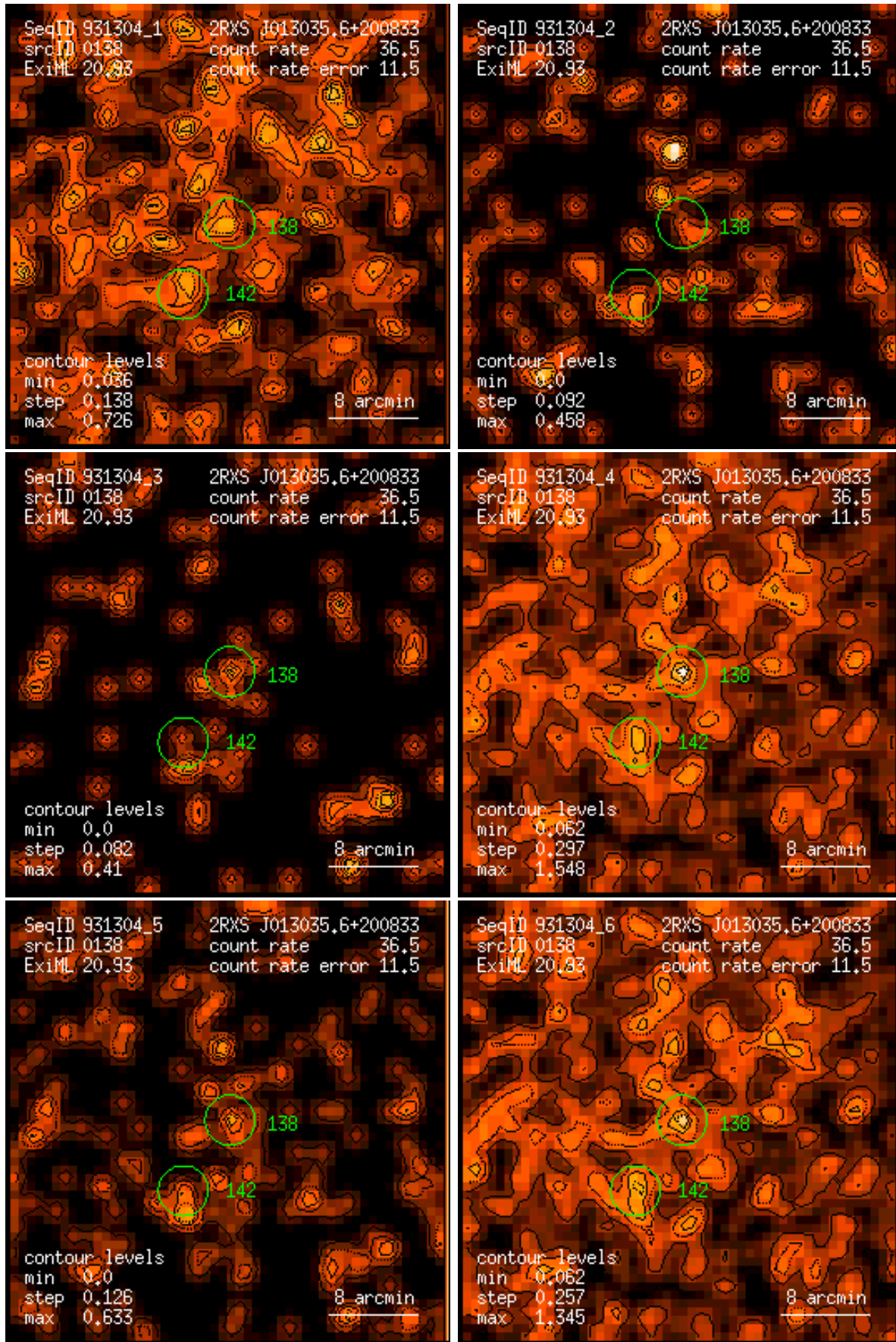
Figure 138: RASS 931304: detection 0138: band rate images, Gaussian filter: (1) PSPC channels 11 – 41, (2) 52 – 90, (3) 91 – 201, (4) 11 – 235, (5) 52 – 201, (6) 11 – 201. Broad band rates in counts/ks. Band rate contour levels in counts/ks/arcmin 2 .
