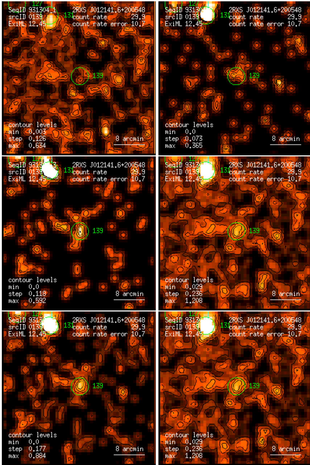
Figure 139: RASS 931304: detection 0139: band rate images, Gaussian filter: (1) PSPC channels 11 – 41, (2) 52 – 90, (3) 91 – 201, (4) 11 – 235, (5) 52 – 201, (6) 11 – 201. Broad band rates in counts/ks. Band rate contour levels in counts/ks/arcmin 2 .
