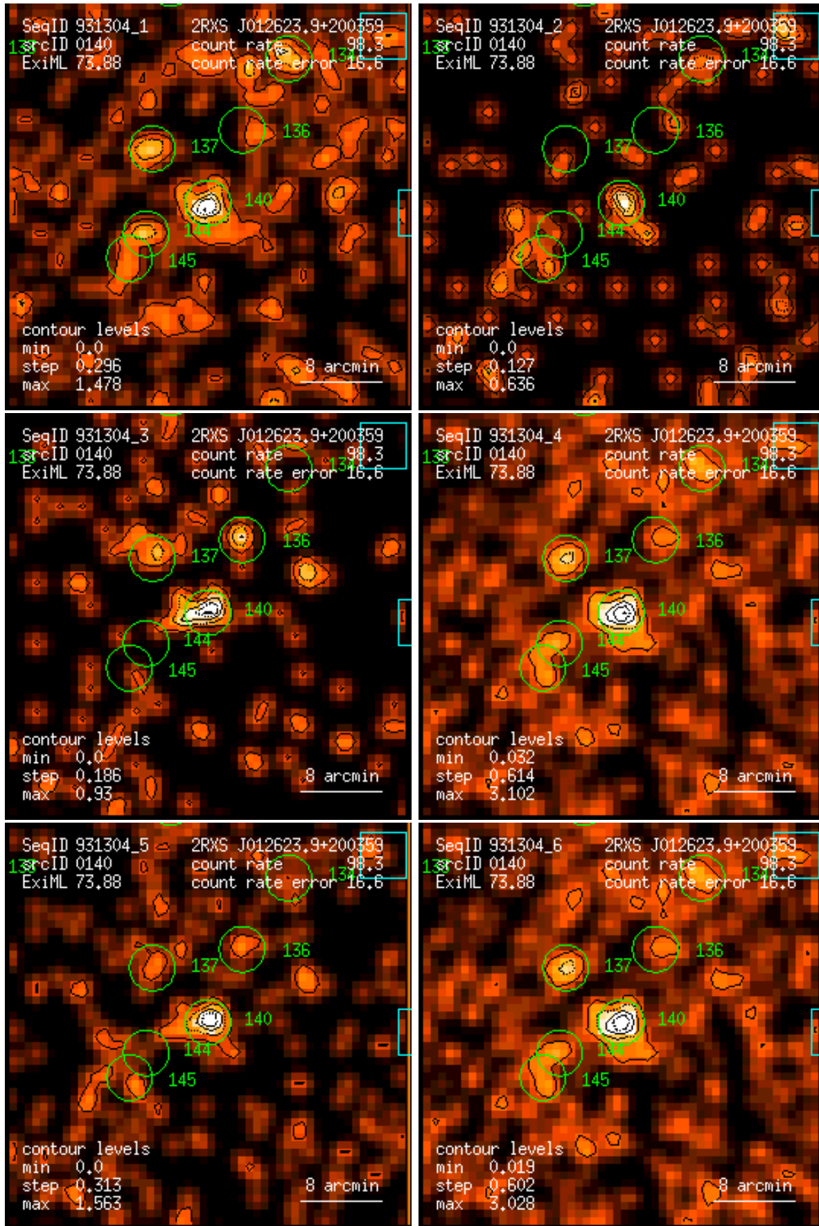
Figure 140: RASS 931304: detection 0140: band rate images, Gaussian filter: (1) PSPC channels 11 – 41, (2) 52 – 90, (3) 91 – 201, (4) 11 – 235, (5) 52 – 201, (6) 11 – 201. Broad band rates in counts/ks. Band rate contour levels in counts/ks/arcmin 2 .
